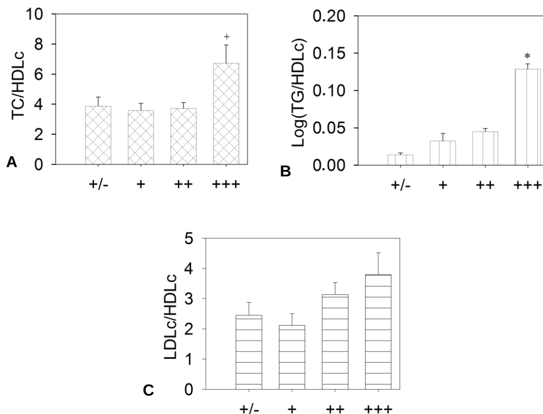
Figure 3. Smear positivity extent variation with atherogenic indices. Changes in atherogenic indices are represented according to the results of SPE scores in TB patients before treatment. The results are presented as mean \pm SEM of atherogenic indices value within SPE scores groups. (+ p <0.01, * p <0.05), (+/-, n = 15; +, n = 16; ++, n = 34; +++, n = 18).
