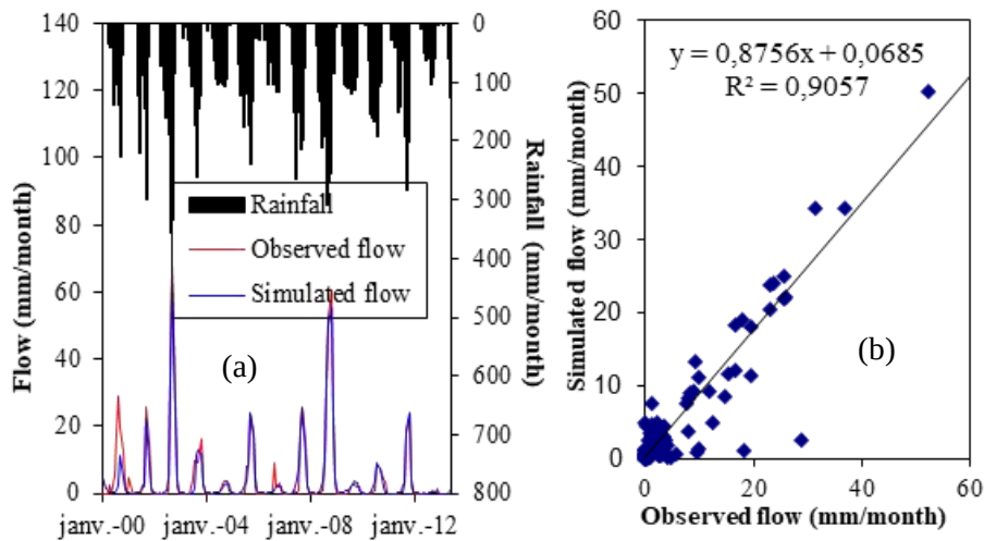
Figure 4 : Validation of the obtained GR2M model from the Bétérrou station: (a) Rainfall-flow based on GR2M model. (b) Correlation from observed vs simulated flows.
