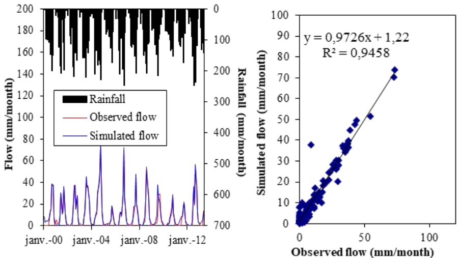
Figure 6 : Validation of the obtained GR2M model at Savè station: (a) Rainfall-flow based on GR2M model. (b) Correlation from observed vs simulated flows.
