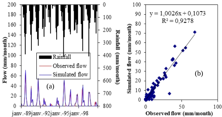
Figure 3 : Blocking of the obtained GR2M model from the Bétérrou station: (a) Rainfall-flow based on GR2M model. (b) Correlation from observed vs simulated flows.
