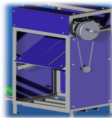
Fig. 1: The Proposed Coconut Stripper.
