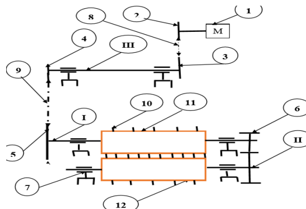
Fig. 2: Kinematic Chain of the Coconut Stripper.
