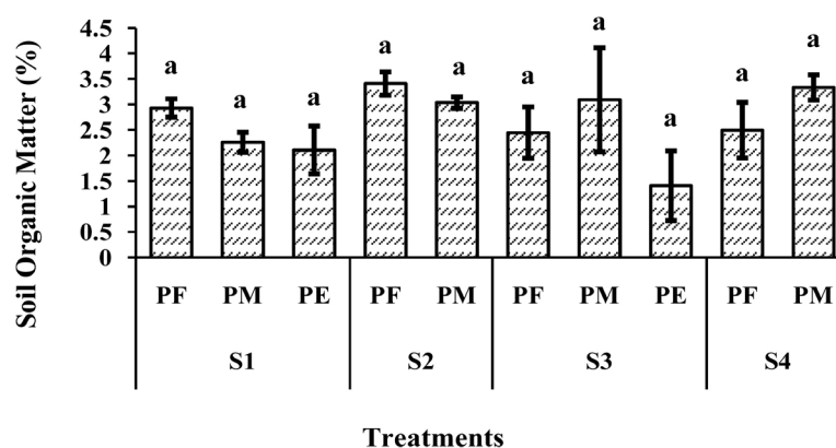
Figure 8. Interactive effect of cropping systems and slope on soil organic matter content. S1: Maize-Cassava; S2: Pure Palm grove; S3: Palm grove-Maize-Cassava; S4: Teak plantation; PF: Low slope; PM: Moderate slope; PE: High slope; histograms bearing the same letter are not significantly different at the 5% threshold.
