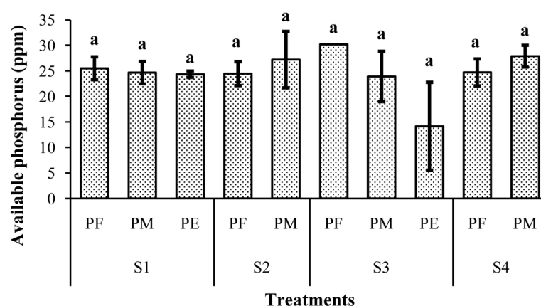
Figure 9. Interactive effect of cropping systems and slope on available phosphorus in the soil. S1: Maize-Cassava; S2: Pure Palm grove; S3: Palm grove-Maize-Cassava; S4: Teak plantation; PF: Low slope; PM: Moderate slope; PE: High slope; histograms bearing the same letter are not significantly different at the 5% threshold.
