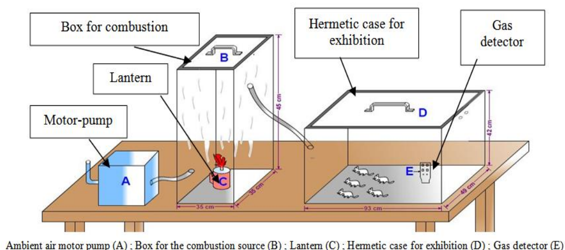
Fig 1: Device used to produce pollutants (CO and NO 2 ) and oxygen (O 2 )
