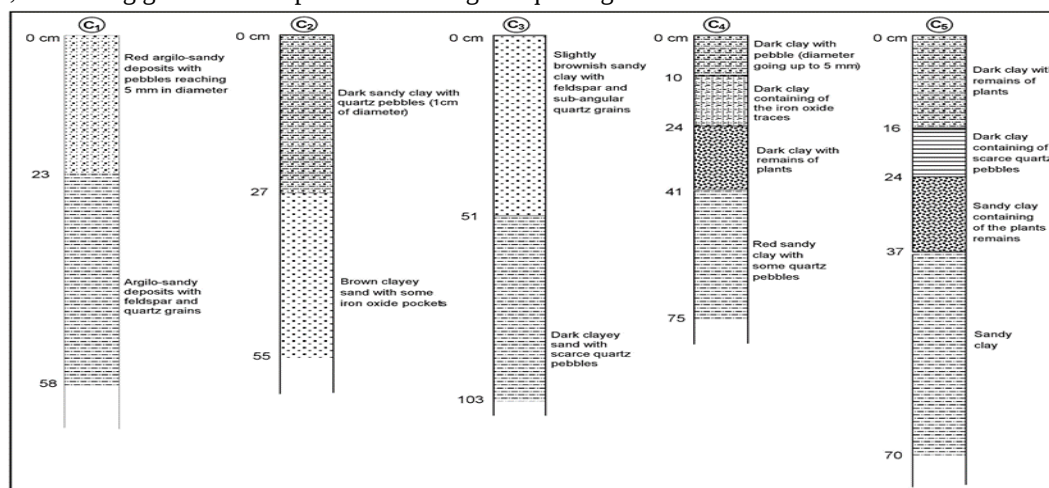
Figure 4: Boreholes logs realized at the edge of Okpara dam
