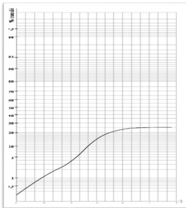
Figure 5: Cumulative granulometric curve of the sediment of station 7
