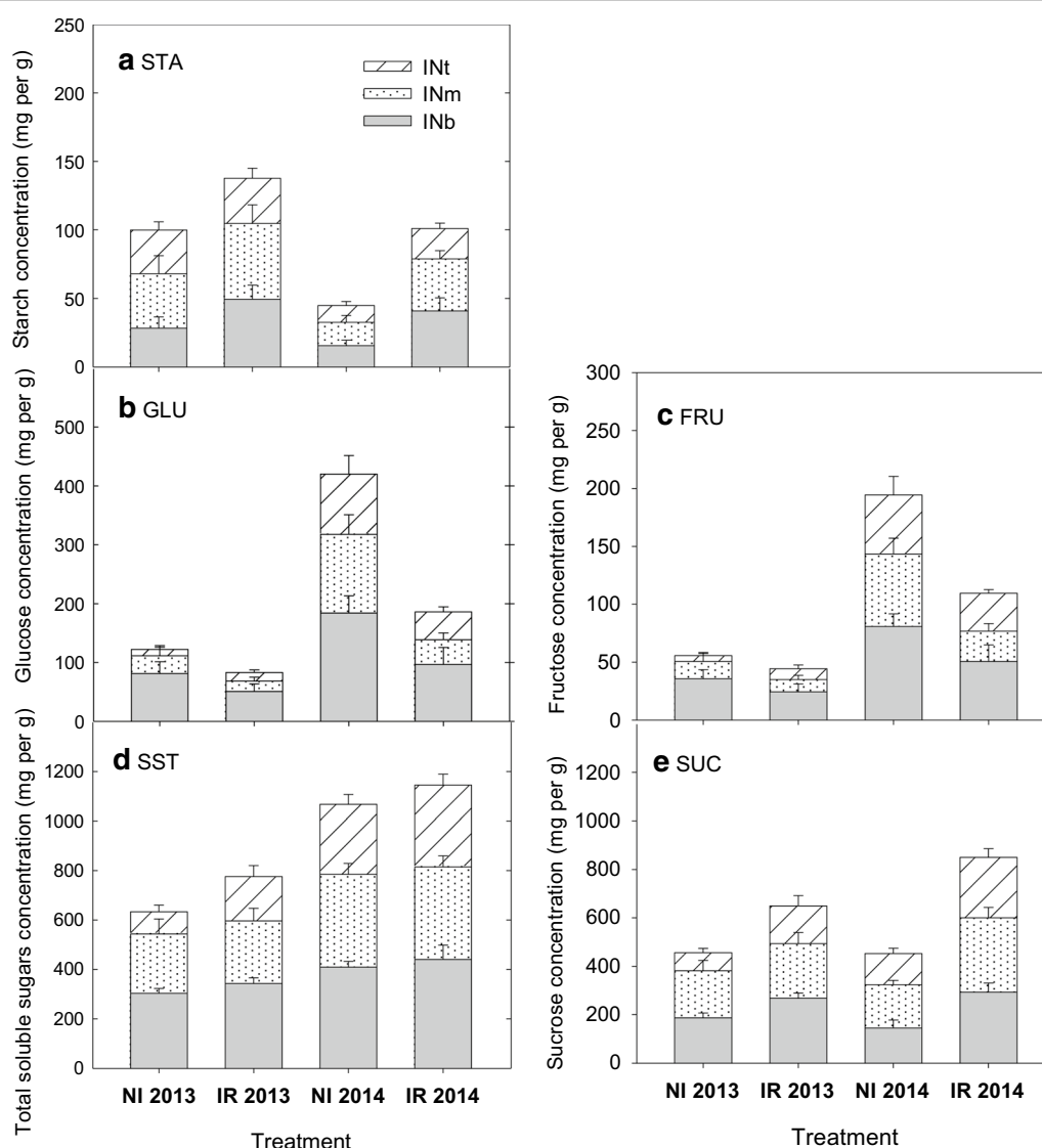
Fig. 4 Carbohydrates (SST: total soluble sugars, SUC: sucrose, GLU: glucose, FRU: fructose and STA: starch) content ( \text{mg g}^{-1} ) compared among stem internodes (INb: bottom, INm: median, INt: top) and water treatments (NI, IR) in 2013 and 2014. Data are average value with standard error of the 4 studied accessions (G3, G7, G10, G11)
