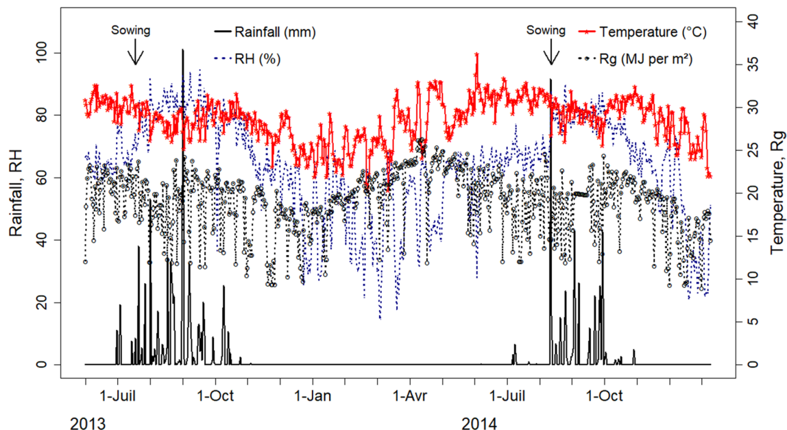
Fig. 1 Daily weather conditions at Bambey station from June 1st, 2013 to December 31st, 2014. Average temperature, average relative humidity (RH), global radiation (Rg) and daily rainfall
