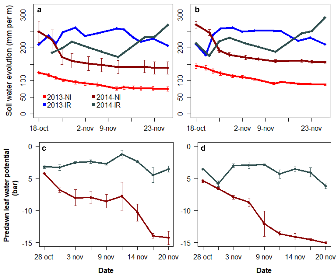
Fig. 2 Post-anthesis soil water content in each water treatment (NI: non irrigated, IR: irrigated) in 2013 and 2014 for the reference accessions SS6 (a) and SS8 (b) and predawn leaf water potential measured during post-anthesis drought in 2014 for SS6 (c) and SS8 (d) reported in Tovignan et al. (2016). Presented data are average value with standard error
