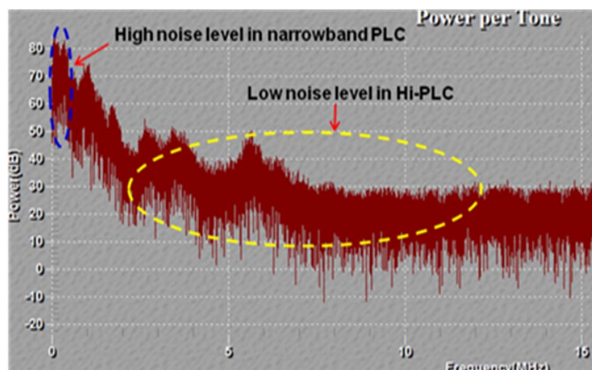
Fig. 7. Noise distribution on the low voltage power line in Residential Area Phase 2 point 2
