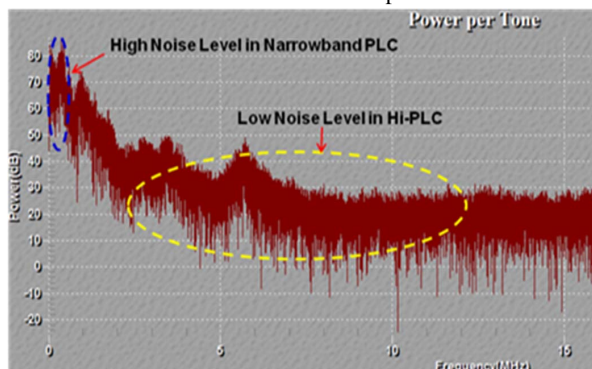
Fig. 6. Noise distribution on the low voltage power line in Residential Area Phase 1 point 1
