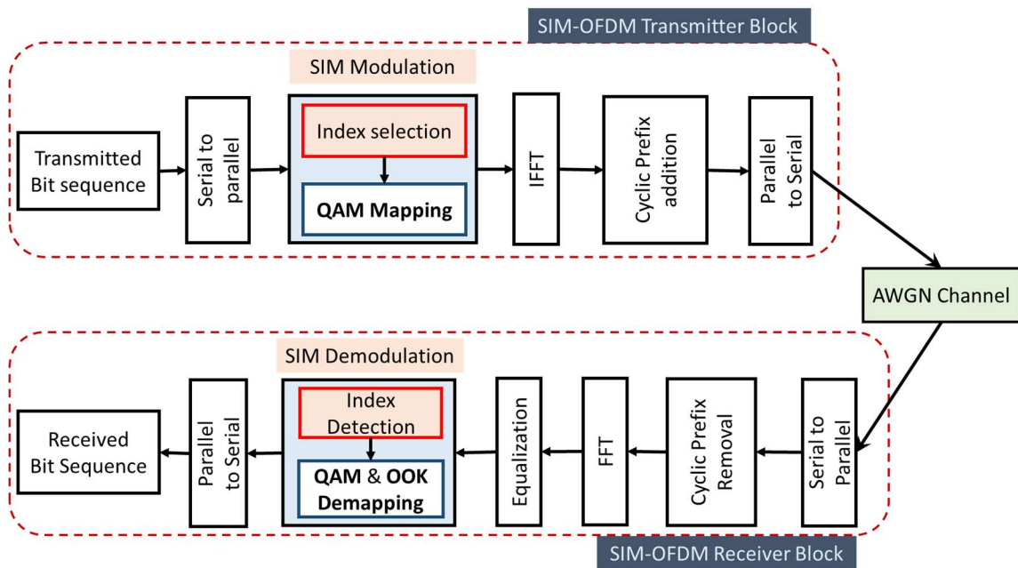
Fig. 2. Block diagram of a SIM-OFDM link under AWGN.
