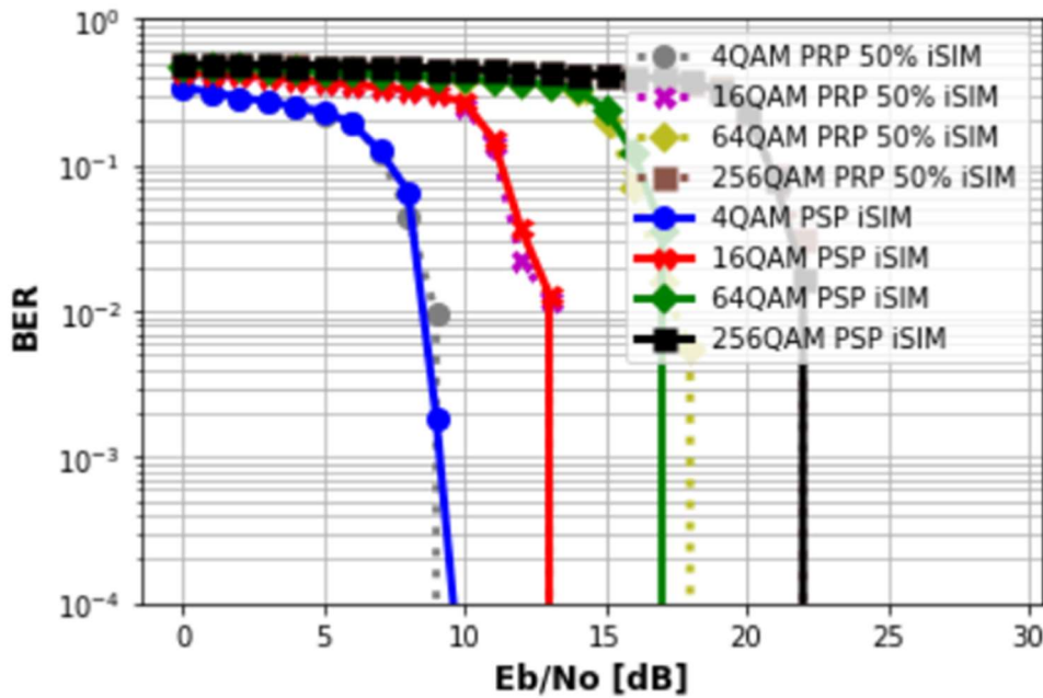
Fig. 4. BER against E_b/N_0 , for improved SIM-OFDM under PSP and PRP when PRP uses 50% of the PSP emitted power for different constellation sizes.
