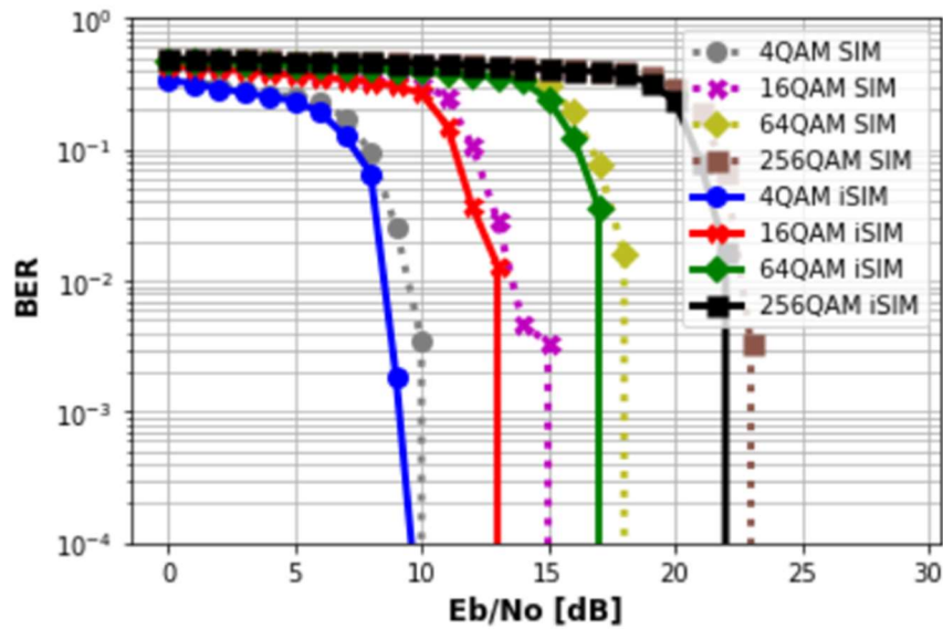
Fig. 3. BER against E_b/N_0 , for improved SIM-OFDM and conventional SIM-OFDM under Power Saving Policy and different constellation sizes.
