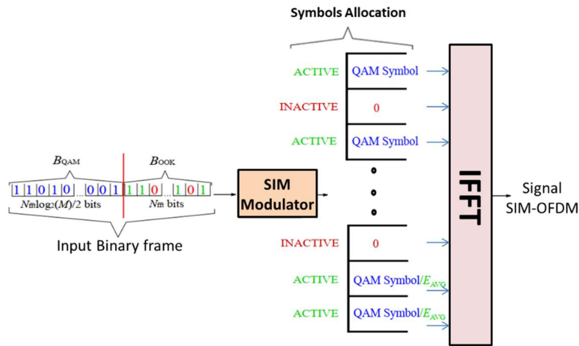
Fig. 1. Principle of SIM-OFDM modulation [8].
