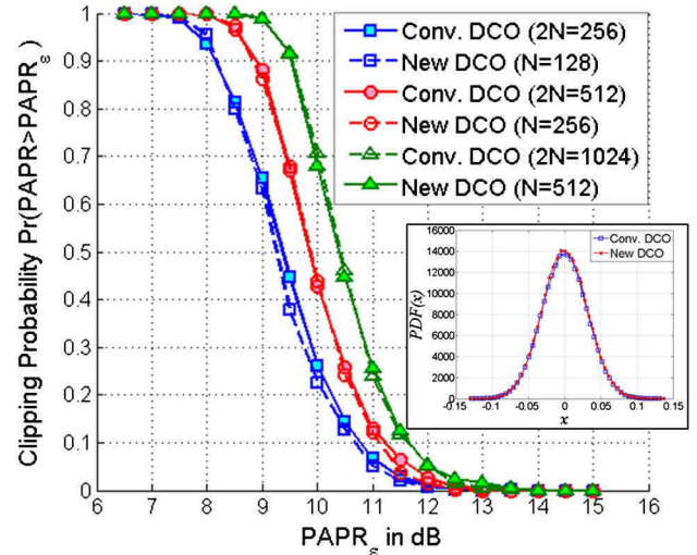
Fig. 5. CCDF comparison of conventional DCO-OFDM and New DCO-OFDM for different (I)FFT sizes. A PDF function of both conventional and New DCO-OFDM signals is shown for easier interpretation.
