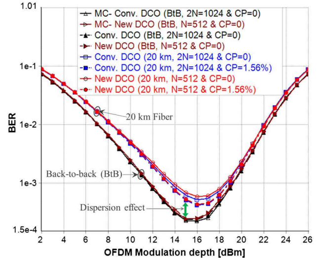
Fig. 9. BER versus modulation depth (OFDM signal power) of the conventional and New DCO-OFDM schemes in back-to-back (without dispersion) and 20 km fiber span at an optical budget of 28 dB and 4QAM constellation. A MC simulation is shown in back-to-back (BtB) for comparison with the theoretical method of Eq. (22).
