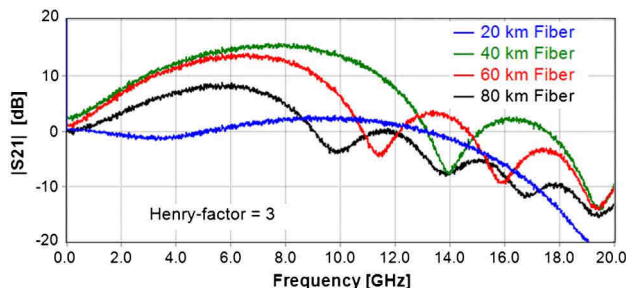
Fig. 1. Channel frequency response variation versus fiber length of the simulated link considering a DFB laser Henry factor of 3.
