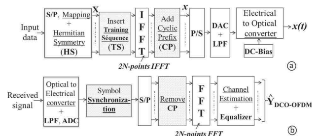
Fig. 2. Block diagram of a conventional DCO-OFDM scheme: (a) transmitter and (b) receiver.
