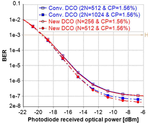
Fig. 11. BER versus received optical power and FFT size of the conventional and New DCO-OFDM signals for 4QAM constellation and 20 km fiber span.
