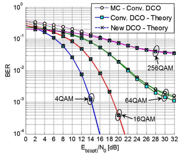
Fig. 8. BER performance versus E_{b(\text{opt})}/N_0 of the conventional DCO-OFDM (Conv. DCO, (I)FFT size of 1024) and the New DCO-OFDM (New DCO, (I)FFT size of 512) for different QAM constellations using theoretical BER calculation. A MC error counting simulation is carried out for conventional DCO.
