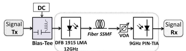
Fig. 7. Simulated IM/DD PON link.
