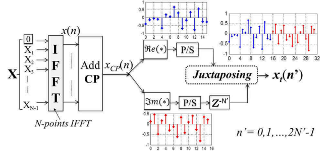
Fig. 3. Transmitter block diagram of the proposed technique including an example of real with imaginary signals and overall transmitted time signal x_t(n') .
