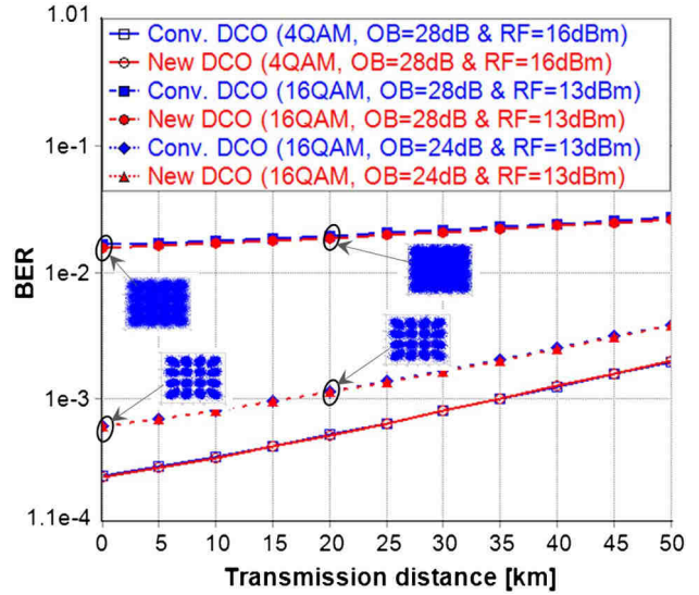
Fig. 13. BER versus transmission distance of the conventional and New DCO-OFDM signal for 4/16QAM constellations with specific optical budget (OB) and optimized RF power values at 2N = 1024 and CP = 1.56\% .
