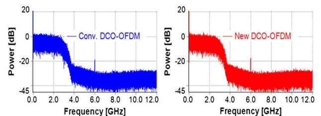
Fig. 10. RF spectrum in the positive side band of the conventional and New DCO-OFDM signals for 4QAM constellation, 20 km fiber span, and optical budget of 28 dB.
