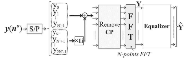
Fig. 4. Receiver block diagram of the New DCO-OFDM.
