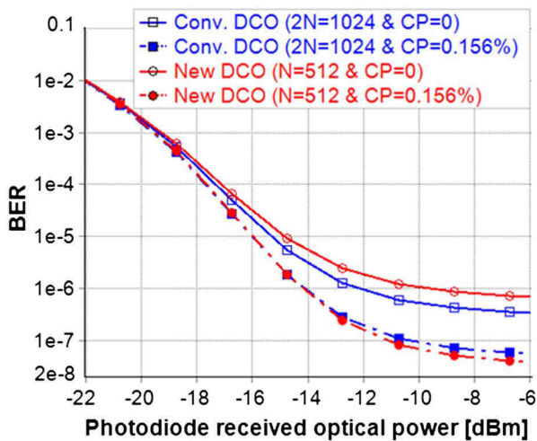
Fig. 12. BER versus received optical power and CP size of the conventional and New DCO-OFDM signals for 4QAM constellation and 20 km fiber span.
