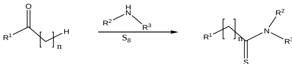
Scheme. 1: Willgerdt-Kindler's reaction.
