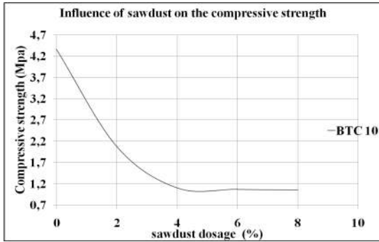
Fig. 5. Influence of dosage of Afzalia sawdust on the resistance in compression
