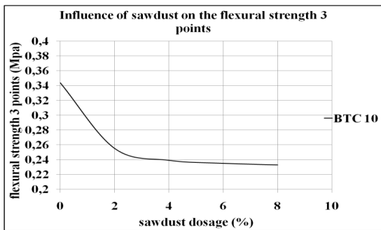
Fig. 6. Influence of dosage of Afzalia sawdust on the resistance in three points flexion
