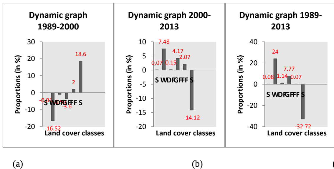
Figure 3: Land cover dynamics from 1989 to 2013 at the hunting zone of Djona (WBR)
