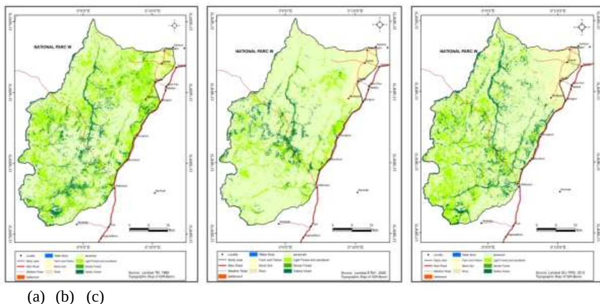
Figure 2: Land covers maps for 1989 (a), 2000 (b) and 2013 (c).
