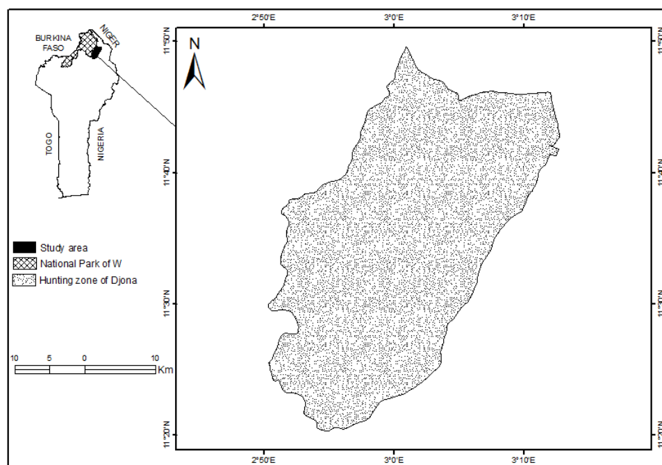
Figure 1: Localization of the study site, the hunting zone of Djona-part of the W Biosphere Reserve (Benin).
