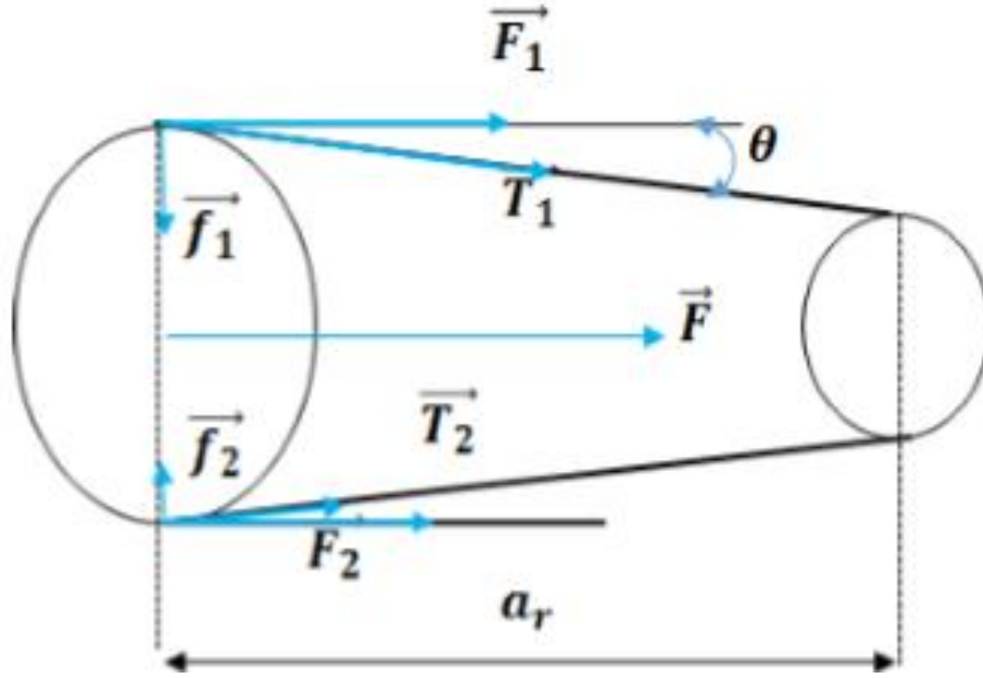
Figure 4: Tension forces 10
