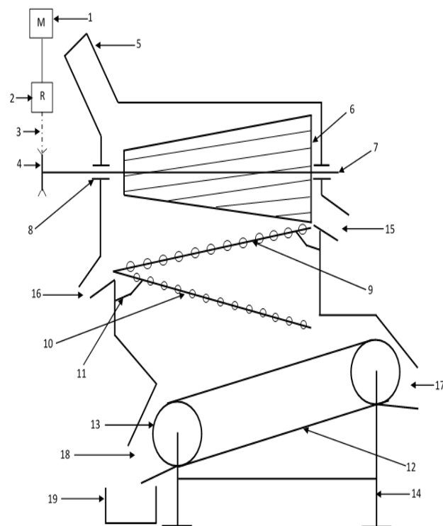
Figure-3: Schematic of the operating principle.
