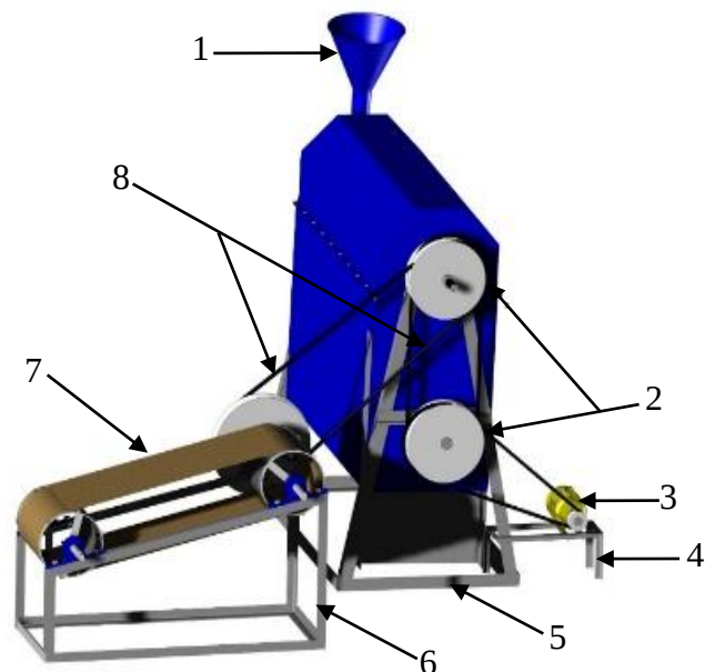
Figure- 1: Proposed separating machine
