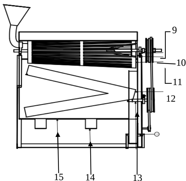
Figure 2: Cross-sectional representation of the separating machine.
