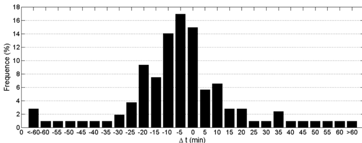
Fig. 8. Frequential spreading of temporal scales between the electrical activity maxima and precipitations for a fixed radius of 5 km around the location of the rain gauges for the overall rainfall events studied.
