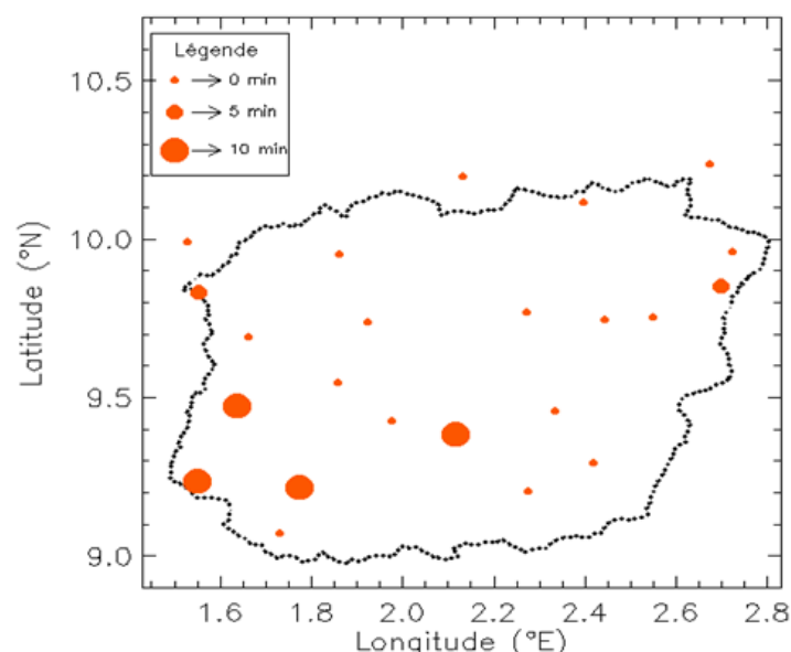
Fig. 5. Time lag between the beginning of electrical activity and precipitation corresponding to the maximal determination coefficient obtained on each rain gauge of the network.
