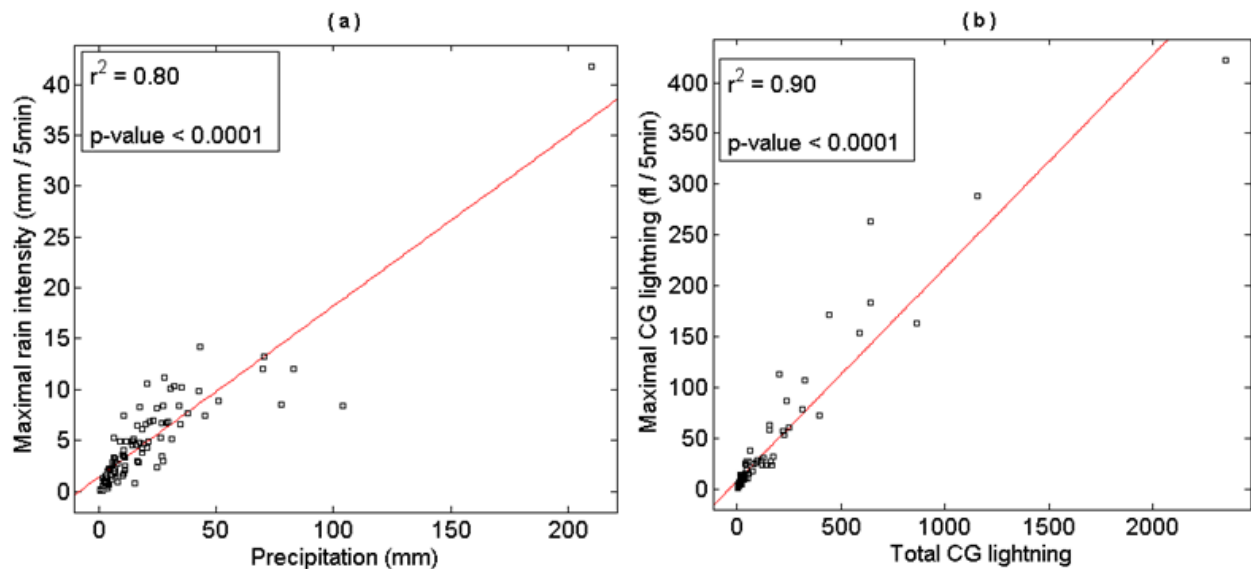
Fig. 4. (a) Correlation between the maximal rain intensity and the total cumulous per rainfall event for the whole selected events; (b) correlation between the maximal rate of CG lightning and the total CG lightning per rainfall event for a 5 km radius around the position of rain gauges.
