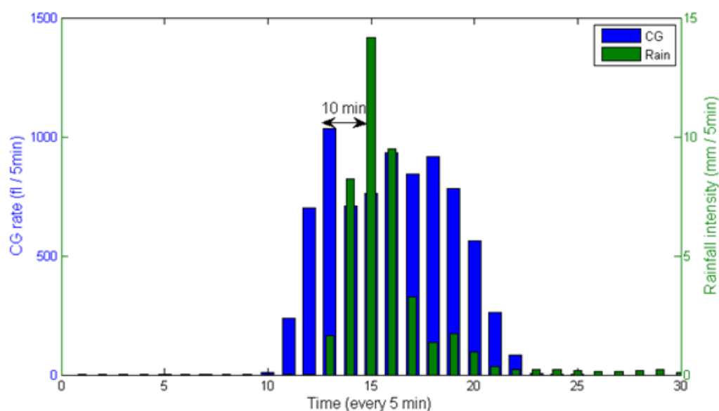
Fig. 3. Temporal evolution of lightning rates and rain intensity show time lag between the maximum CG lightning and precipitation observed at the meteorological station of Djougou during event n°2 (table 1).
