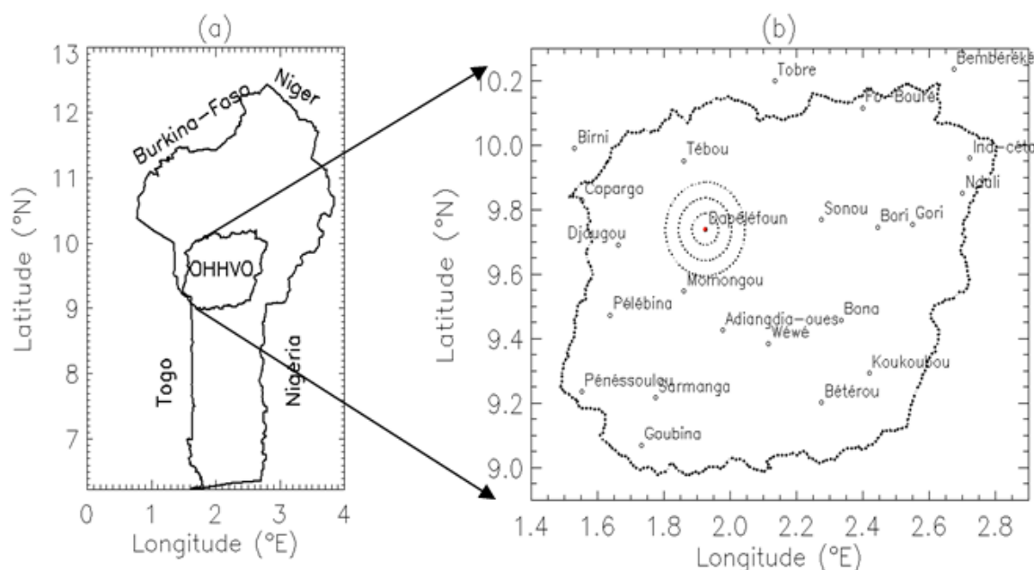
Fig. 1. (a) Geographical situation of Benin with the boundaries of the OHHVO, (b) sub-network composed of twenty three rain gauges used for the study.
