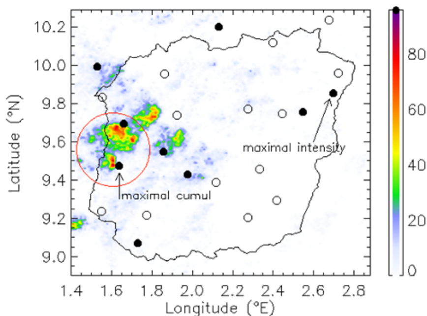
Fig. 6. Cloud-to-ground lightning density map corresponding to event n°2. The close circles indicate rain gauges that have had a rain cumulus superior to the average cumulus of the event and the red circle indicates the area that could be considered as stormy area on looking at it lightning density.
