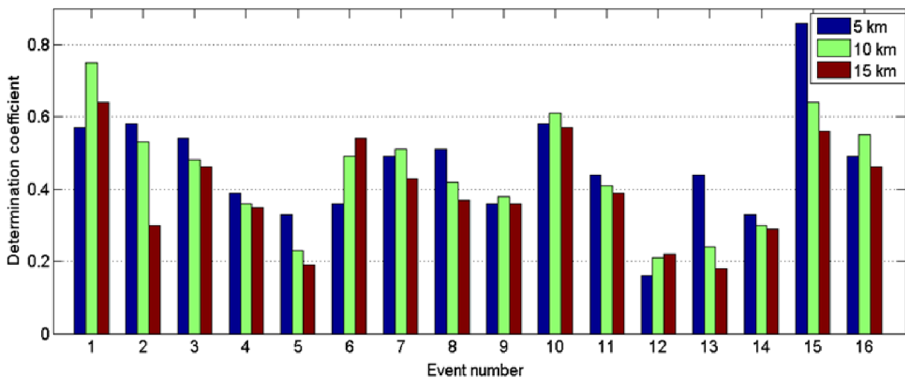
Fig. 7. Average determination coefficients per rainfall event for different values of R when the beginning of electrical activity and precipitations are synchronized.
