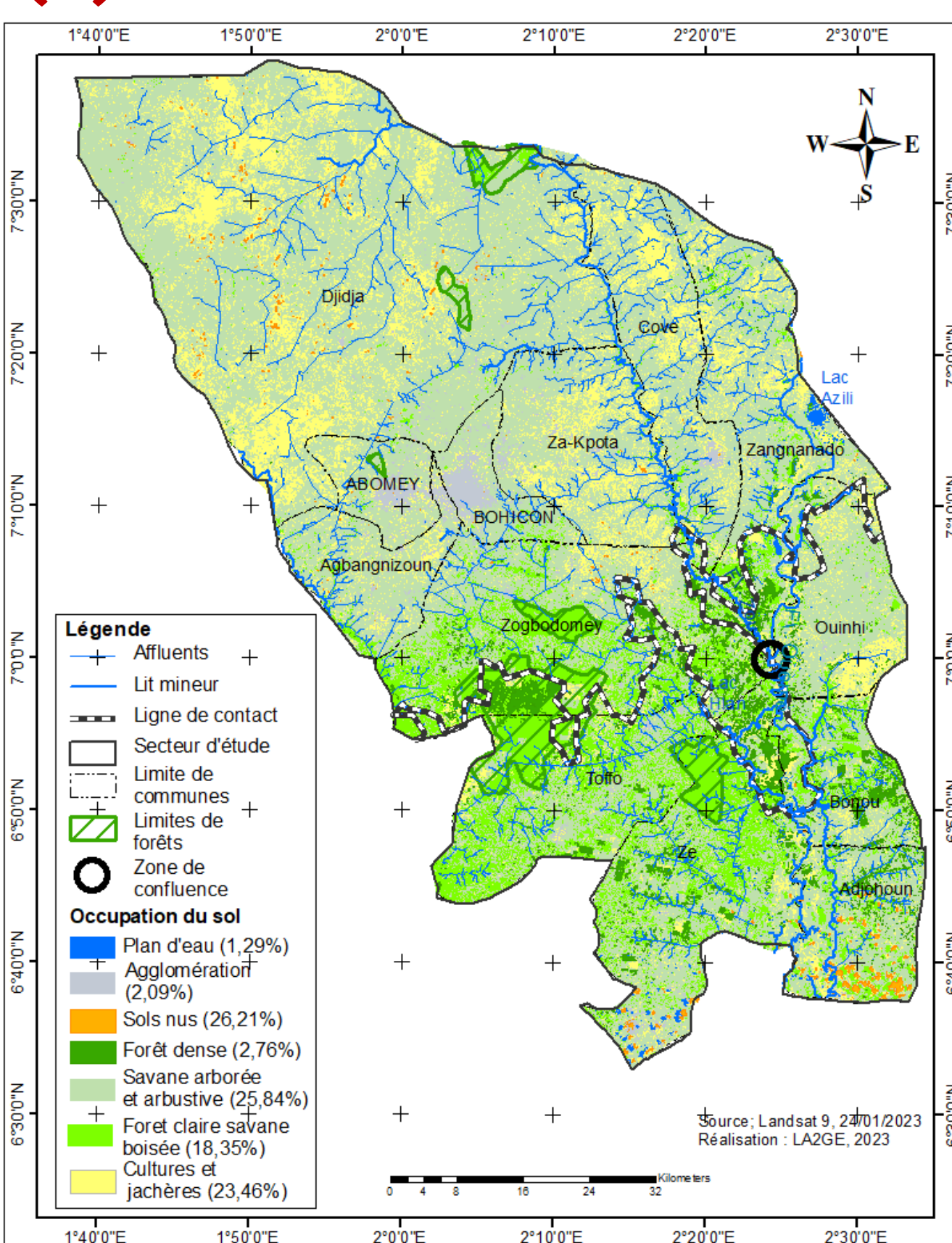
Fig.6: Occupation du sol
