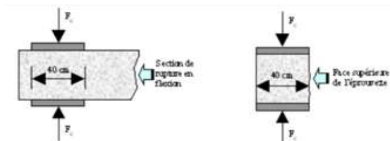
Fig. 2:- Compression fracture device.
