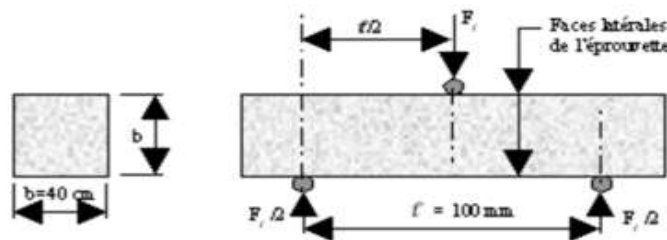
Fig. 1:- System for bending strength test.
