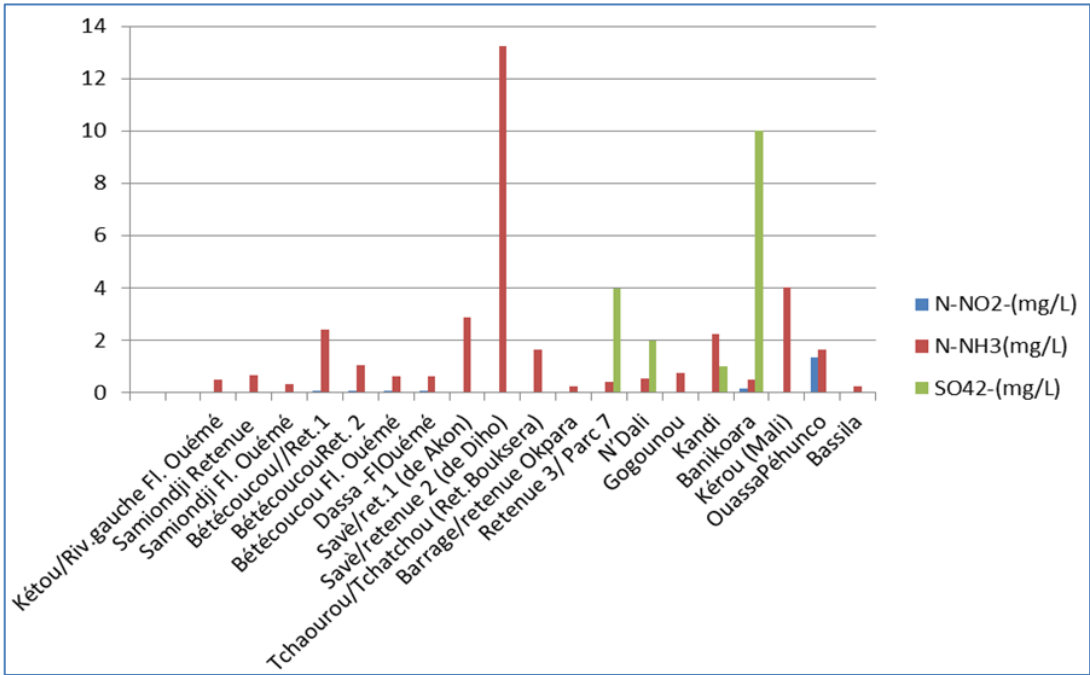
Fig 4: Physico-chemical characteristics of the reservoirs and water bodies of the sites (continuation and end)
