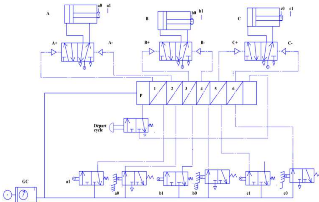
Figure 3: Pneumatic connection circuit
