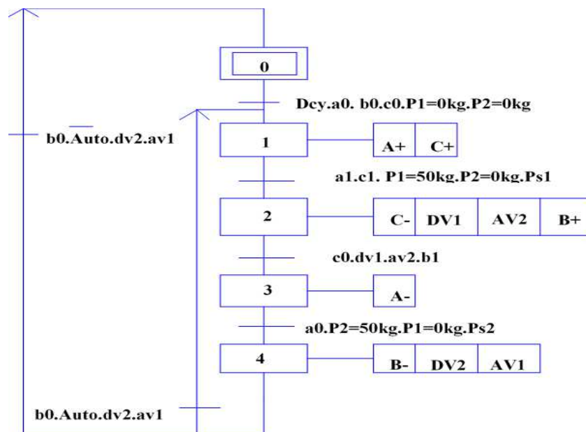
Figure 2: Grafset level II
