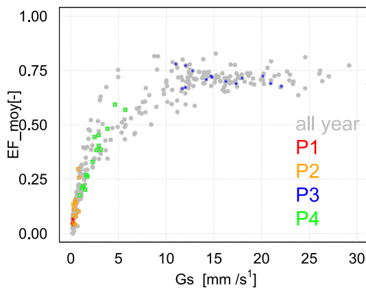
Fig. 11. Midday (10:00–14:00 UTC) evaporative fraction ( EF_{moy} ) versus midday surface conductance ( G_s ) for the whole year (grey) and for the four periods. P1: 18 January–1 February (red); P2: 26 February–11 March (orange); P3: 7–21 July (blue) and P4: 24 October–7 November (green).
