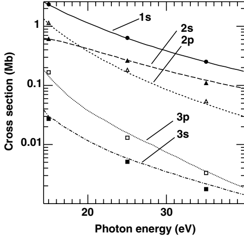
FIG. 3. Partial cross sections for photodetachment of H^- for photon energies above the double-ionization threshold. The residual hydrogen atom is left in its ground state ( 1s ) and various excited states indicated in the figure. The lines correspond to the results obtained with the Proulx-Shakeshaft method. The dots, triangles, and squares at photon energy of 15 eV, 25 eV, and 35 eV are our J -matrix results.
