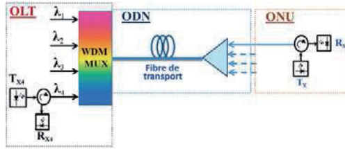
Figure 1.11: Architecture de base du TWDM.
