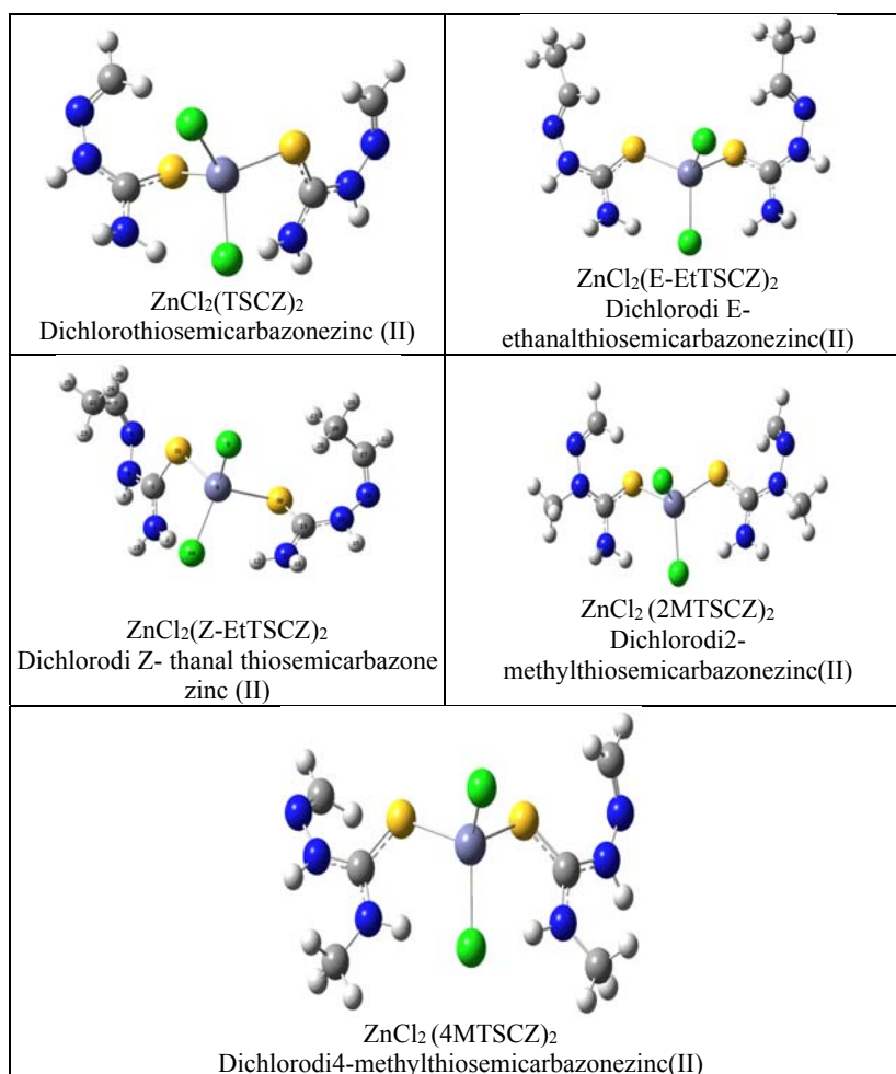
Fig 3: Structure of the complexes \text{ZnCl}_2 \cdot 2\text{Ligand}
