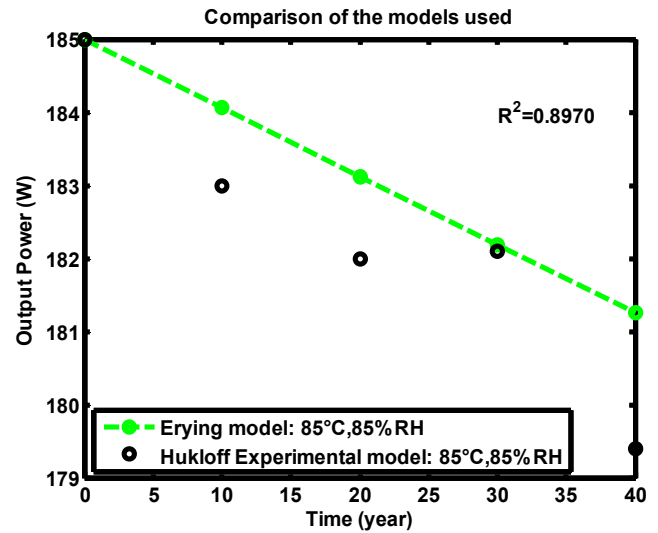
Figure 17. Output power according to time (Erying and Hukloff models).
