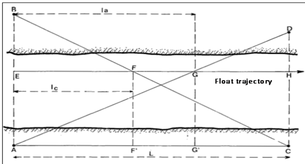
Fig. 1. Determination of the speed of the floats.
