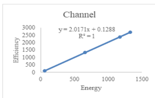
Figure 2: Energy calibration curve
