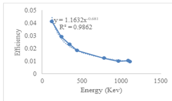
Figure 3: Efficiency calibration curve of the HPGe detector
