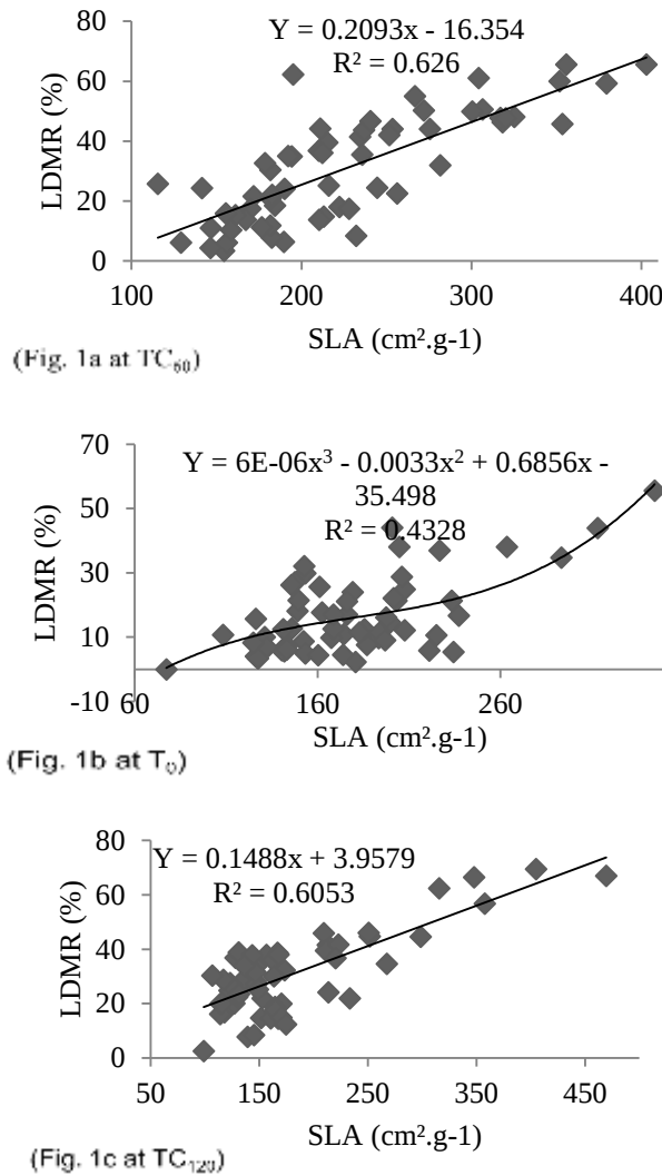
Figure 1. Covariations of SLA with LDMR (N = 180 leaves ; r = 0.88 ; p < 0.01 ). The positive trend was due to the controls that are showed lower values for both traits while the others expressed the highest values.
