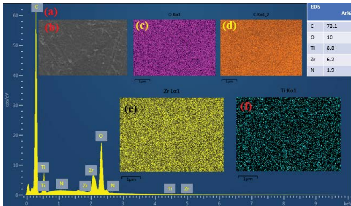
Fig. 2. (a) Energy spectrum analysis results of NF-TiZr 2 :1 membrane and the sample table surface elements containing (b) scanning electron microscopy (SEM) of NF-TiZr 2 :1, (c) oxygen, (d) carbon, (e) zirconium, and (f) titanium.
