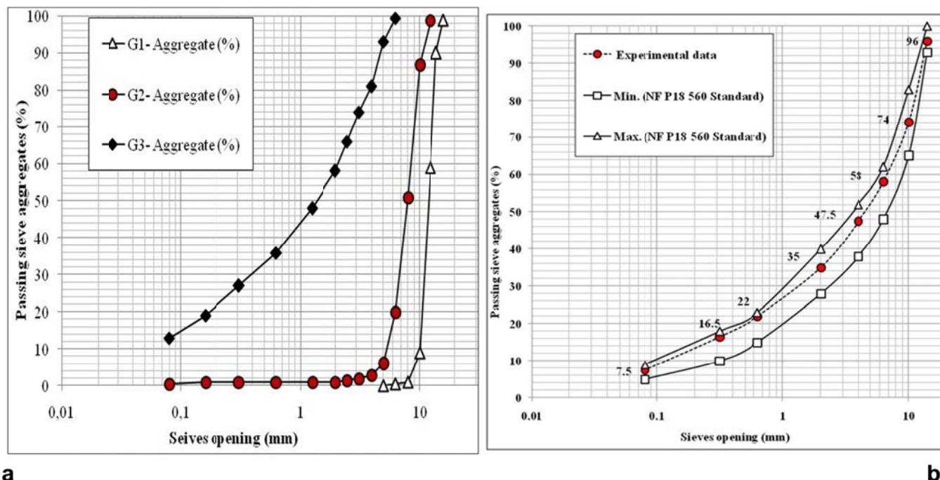
Figure 1. Particles size of the used aggregates and location in relation with the recommendations of NF P18-560 standards (Editions, 1997): two extreme curves a. Particles sizes of aggregates G1, G2 and G31. b. Used aggregate mix particles size.
