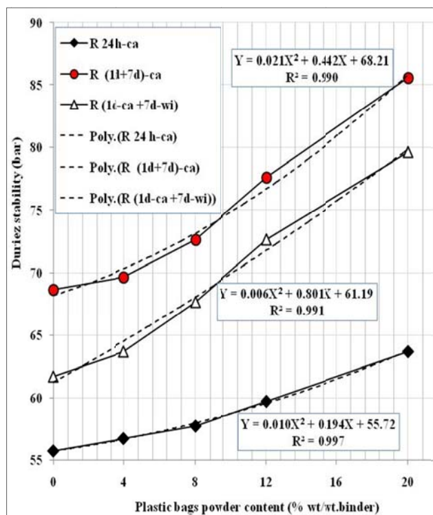
Figure 6. Evolution of Duriez stability of built bituminous concretes versus their molten plastic bags contents: R24h-ca: on the controlled air (c.a) for 24 h; R(1d+7d)-ca: on controlled air (c.a) for 8 days; R(1d-ca+7d-wi): 1-day on controlled air + 7-days water immersed (w.i) at 18°C.
