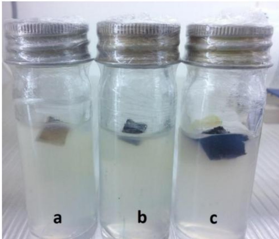
Figure 2 : Browning intensity
