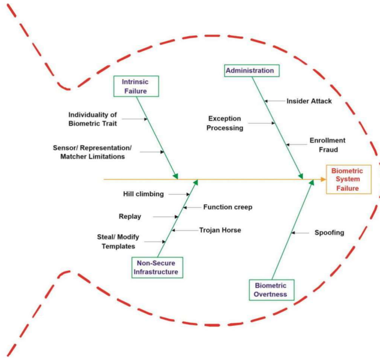
Figure 5: Fish-bone model for categorizing biometric system vulnerabilities [32]
