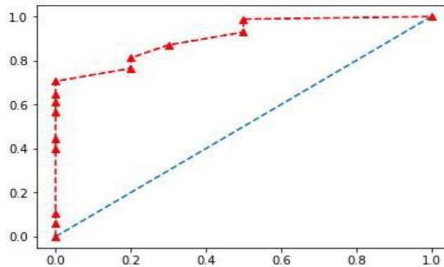
Figure 7: ROC curve with AUC: 0.908
