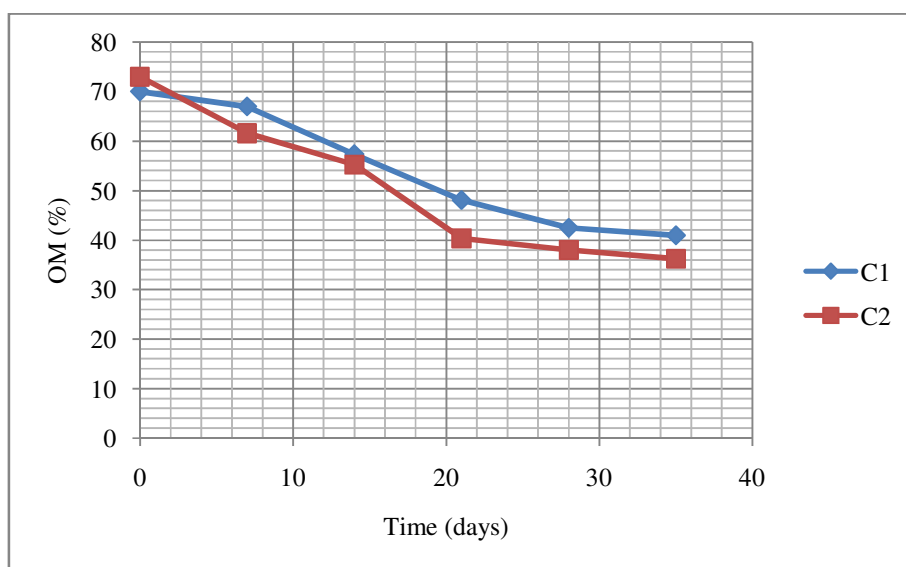
Figure-4 Variation of compost organic matter content during composting
