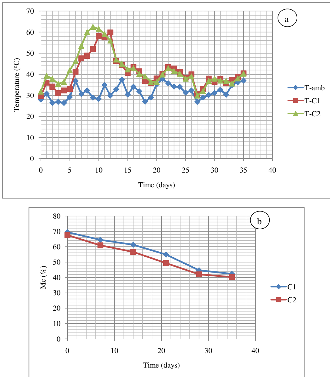
Figure-2 Variation of compost (a) temperature and (b) Moisture content during composting
