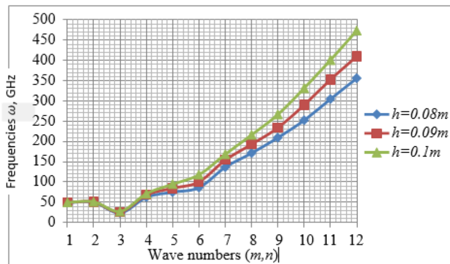
Figure 7. Frequency variation curves based on 12x12m
