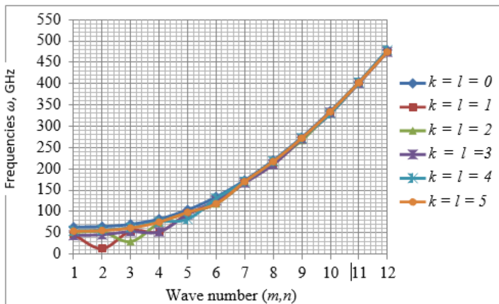
Figure 4. Frequency variation curves based on the wave numbers (m, n) for 8x8m shell
