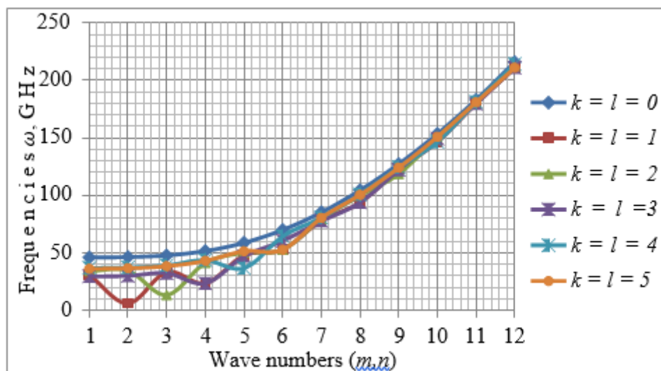
Figure 4. Frequency variation curves based on the wave numbers (m, n) for 8x8m shell
