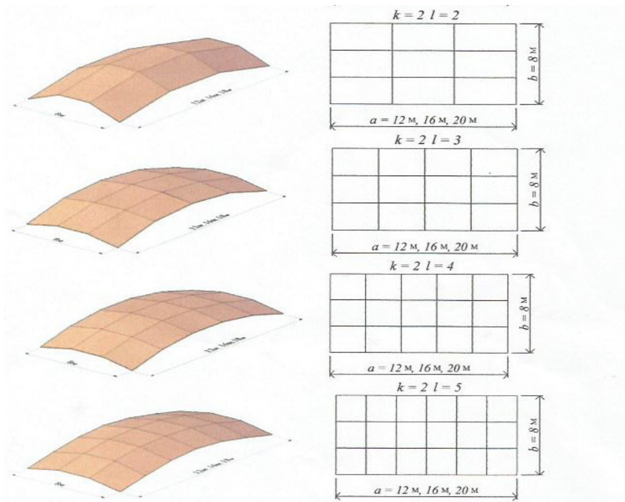
Figure 3. Mathematical models of low rectangular-plan folded shells
