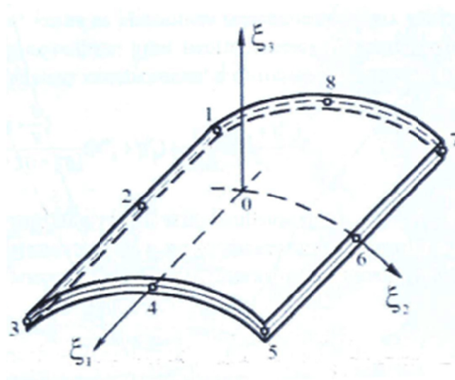
Figure 1. Eight-node iso-parametric curvilinear element
