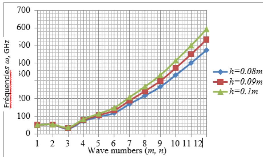
Figure 6. Frequency variation curves based on 8x8m shell thickness
