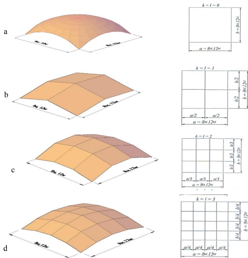
Figure 2. Mathematical models of square-plan low shells
