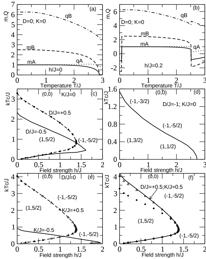
FIG. 6: Thermal behavior of sub-lattice order parameters m and Q at h/J = 0 ; D/J = 0 ; K/J = 0 (a) and h/J = 0.2 and D/J = 0 and K/J = 0 (b). In panel (a), there is a second order phase transition between a ferromagnetic and a paramagnetic phases, whereas in (b) jumps occur in the magnetization showing first order transitions between ordered phases. In panels (c – f), thermal phase diagrams are presented for D/J = \pm 0.5 and K/J = 0 . (c); D/J = -1 and K/J = 0 (d); K/J = \pm 0.5 and D/J = 0 (e) and D/J = K/J = 0.5 (f). Signs in panels (f) are simply added for comparison (see text) and refer to panels (c) and (e): triangles for D/J = 0.5 and K/J = 0 and circles for D/J = 0 and K/J = 0.5 . Phases ( m_A, m_B ) displayed in panels (c) and (e) refer to dash transition lines with positive values of the coupling constants.
