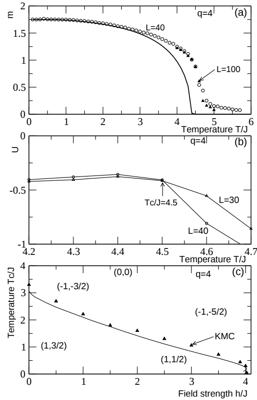
FIG. 7: Compared results by recursion relations (full line) on the Bethe lattice and KMC simulations on a square lattice (signs) of sizes L = 100 and L = 40 for a coordination number q = 4 (panel (a)). In panel (b), a binder crossing point of cumulants U_L(t) calculated for two system sizes L = 40 and L = 30 is shown. This point indicates a transition temperature T_c = 4.5J , which is very close to that obtained by recursion relations. In panel (c), phase diagrams are compared by both methods in the case: D/J = -1.0 , K/J = 0 and q = 4 . Full line shows results by recursion relations, whereas signs indicate simulation results by means of cumulant calculations. Marked agreement between both transition lines appears evident.
