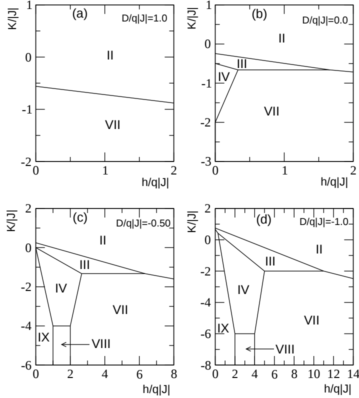
FIG. 5: Ground state phase diagrams for selected values of D/q|J| and varying h/q|J| and K/|J| . The different phases indicated with Roman numbers are explained in Table VI.
