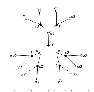
FIG. 1: A Bethe lattice of coordination number q = 3 consisting of two different types of atoms A and B with spin variables S and \sigma respectively.
