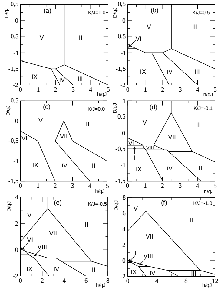
FIG. 4: Ground state phase diagrams for selected values of K/J and varying h/qJ and D/qJ . The different phases indicated with Roman numbers are explained in Table III.
