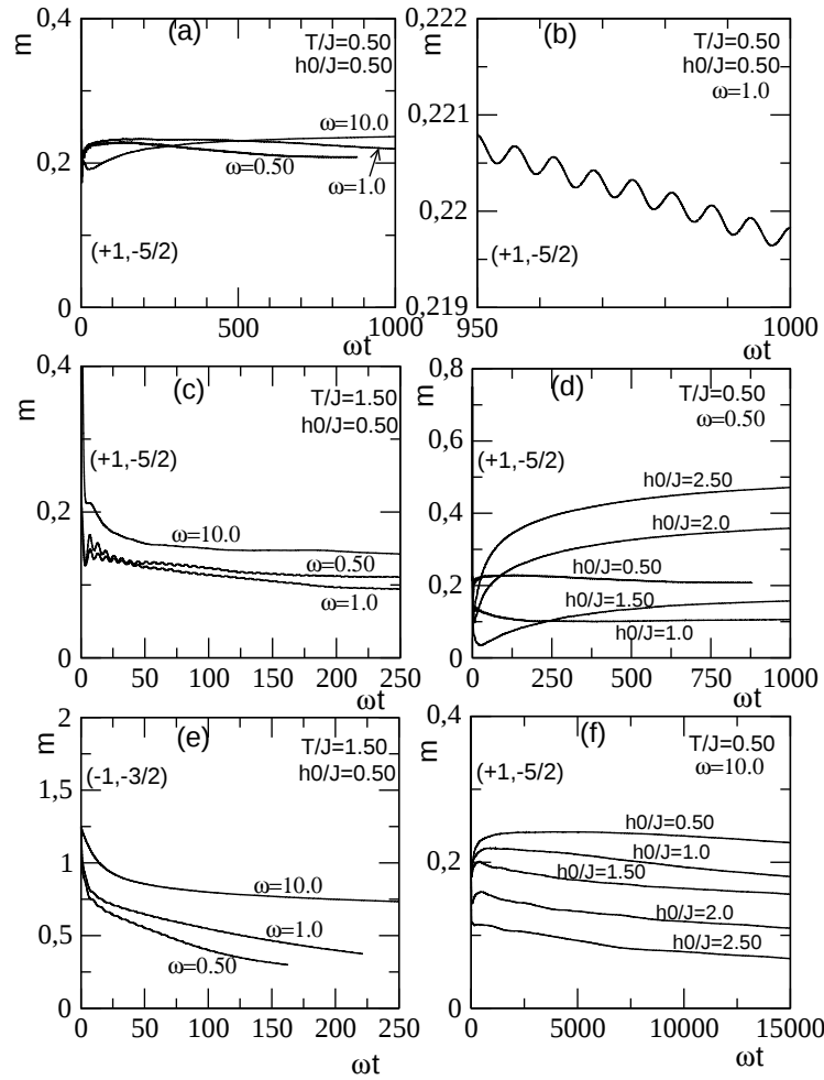
FIG. 8: Time evolution of the lattice total magnetization m(t) were obtained by KMC simulations for a system of size L = 100 . The values of the model parameters considered are written in different panels. In panels (a), (c) and (e), the effect of the field frequency on m(t) is shown for two different GS configurations. On the contrary, in panels (d) and (f), the effect on the amplitude on the stationary behavior of m(t) is investigated for the same initial configuration. Calculations are performed for K/J = -0.5 and D/J = 0 . Behaviors of m(t) with model parameters appear non-trivial.
