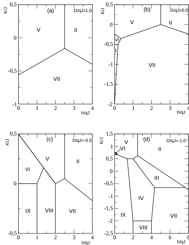
FIG. 3: Ground state phase diagrams for selected values of D/qJ and varying h/qJ and K/J . The different phases indicated by Roman numbers are explained in Table III.
