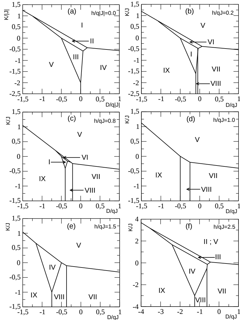
FIG. 2: Ground state phase diagrams for selected values of h/qJ and varying D/qJ and K/J . The different phases indicated with roman numbers are explicated in Table I for h = 0 (panel a) and in Table III for non-zero h/qJ (panels b-f).
