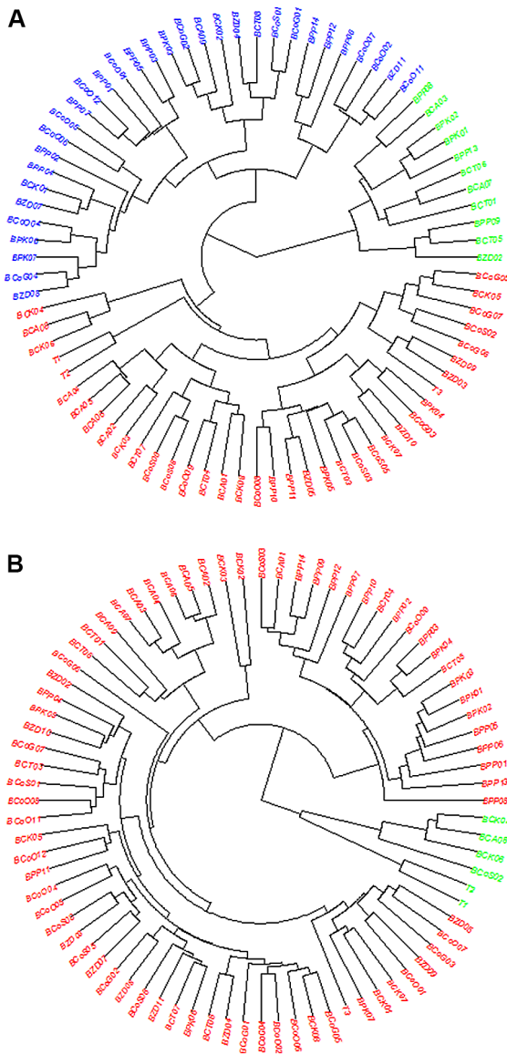
Fig. 6 Phylogenetic trees constructed from a SSR and b SNP data showing the relationships between the 80 Beninese pigeon pea accessions evaluated
