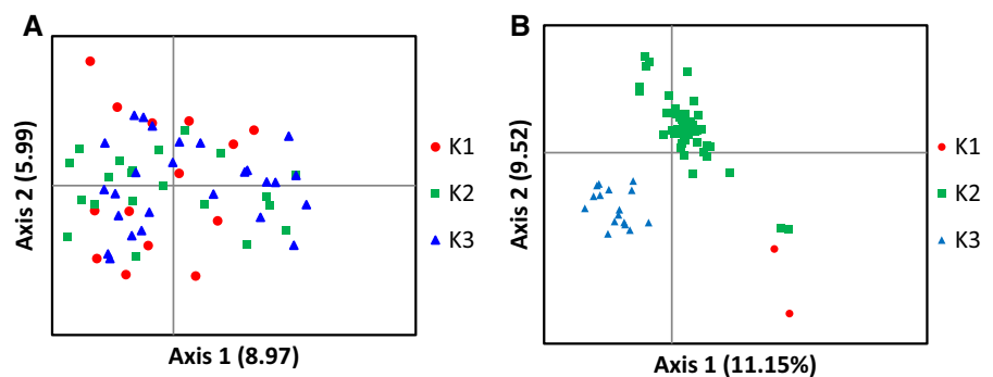
Fig. 5 Principal coordinates analysis showing the divergence within Beninese pigeon pea accessions based on SSR (a) and SNP (b) markers. Individuals with same color belong to the same genetic group
