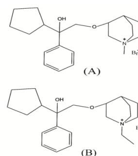
Fig. 1: Chemical structure of BCQB (A) and IS (B)
