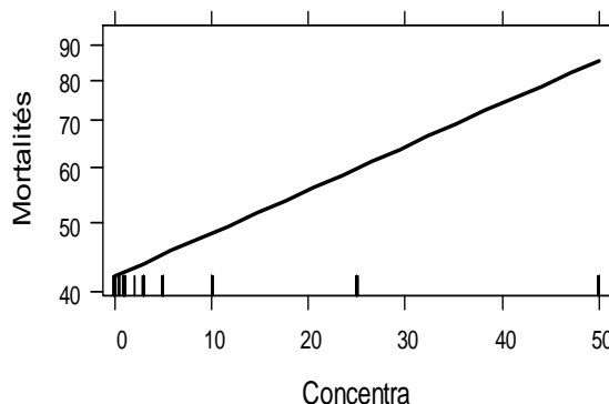
Concentra effect plot
