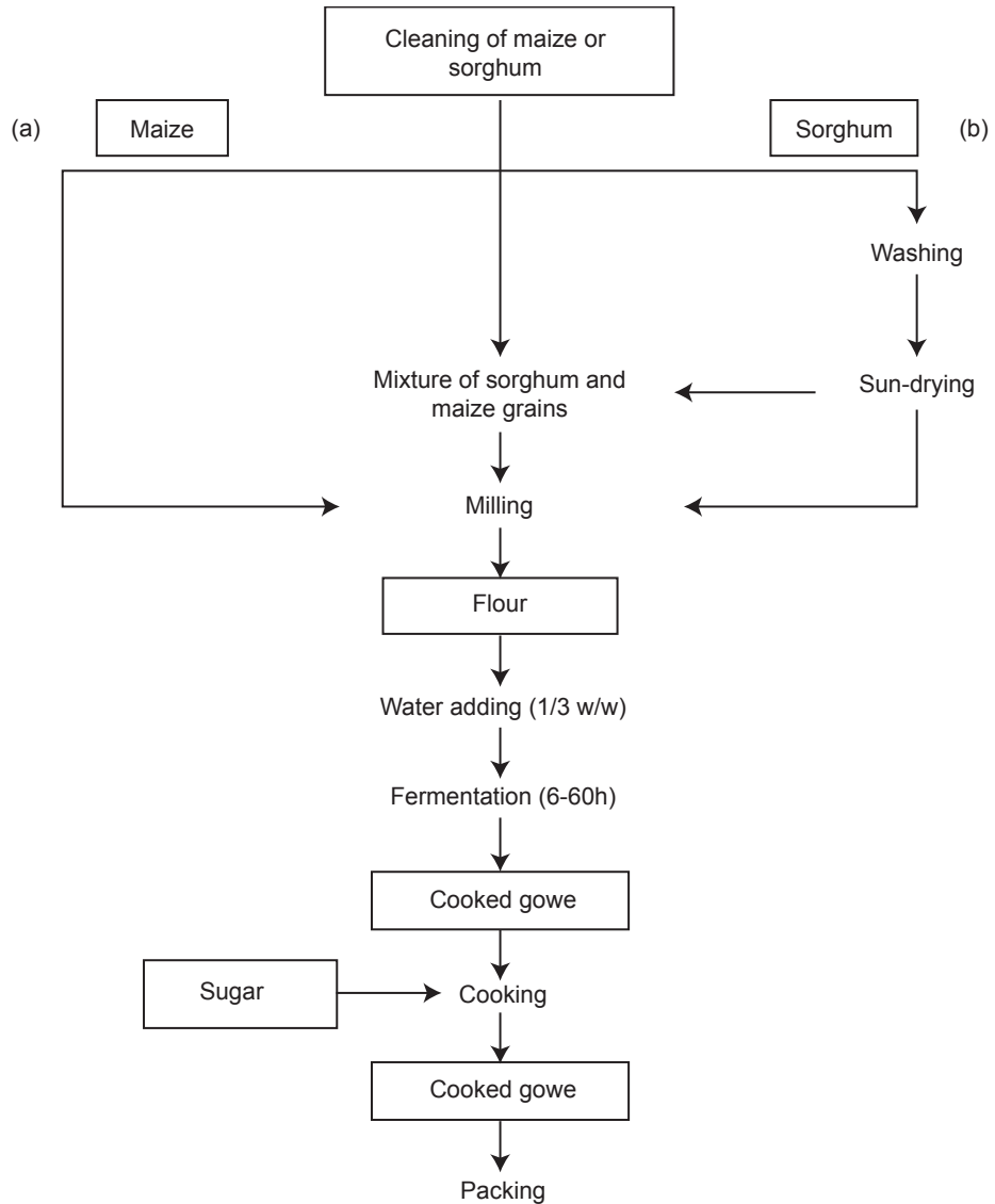
Figure 2 Flow diagram of gowe processing from non-malted grains
