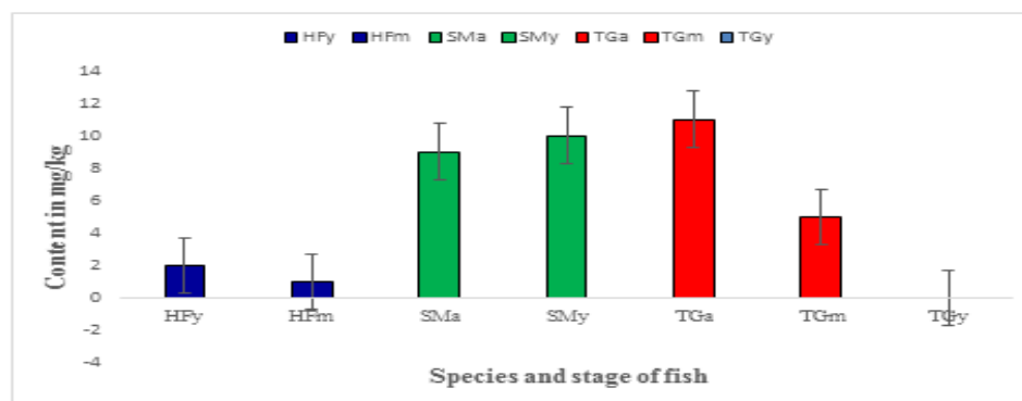
Figure 2. Concentration of lead in the various fish species of Lake Nokoué at different stages of their development.
