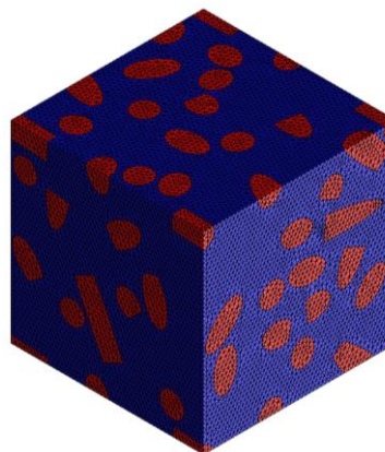
(c) Mesh of the composite Figure 2: RVE meshing
