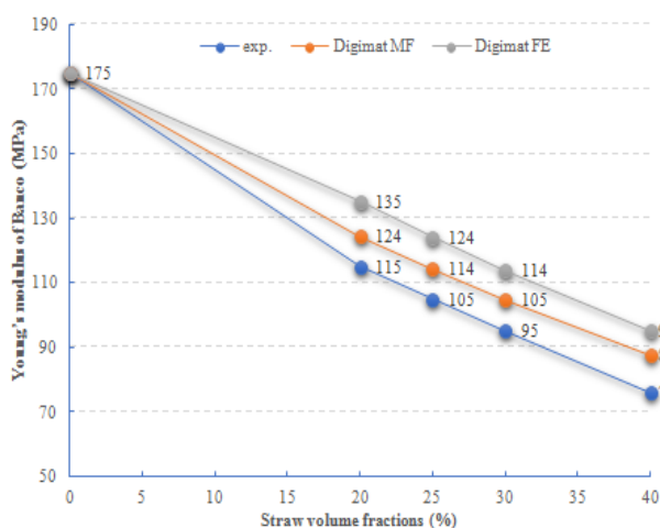
Figure 4: Estimation of the Young's modulus of the Banco composite as a function of the volume fraction of rice straws.
