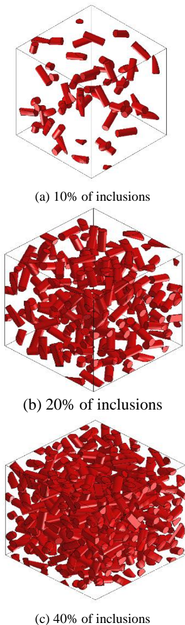
Figure 1: RVE model generated by Digimat code
