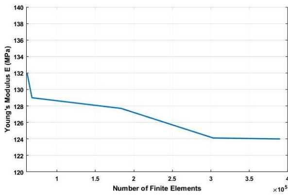
Figure 3: Convergence of the Young's modulus as a function of the number of FE for the different grids of mesh.
