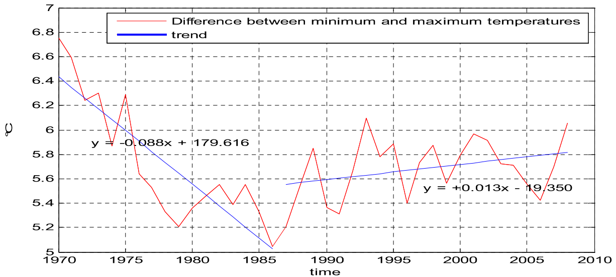
Fig. 5. Evolution of differences between minimum and maximum temperatures in Cotonou: from 1970 to 2008.
