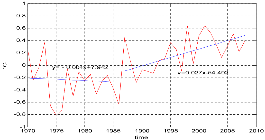
Fig. 2. Change in average annual temperatures and their linear trends in Cotonou between 1970 and 2008
