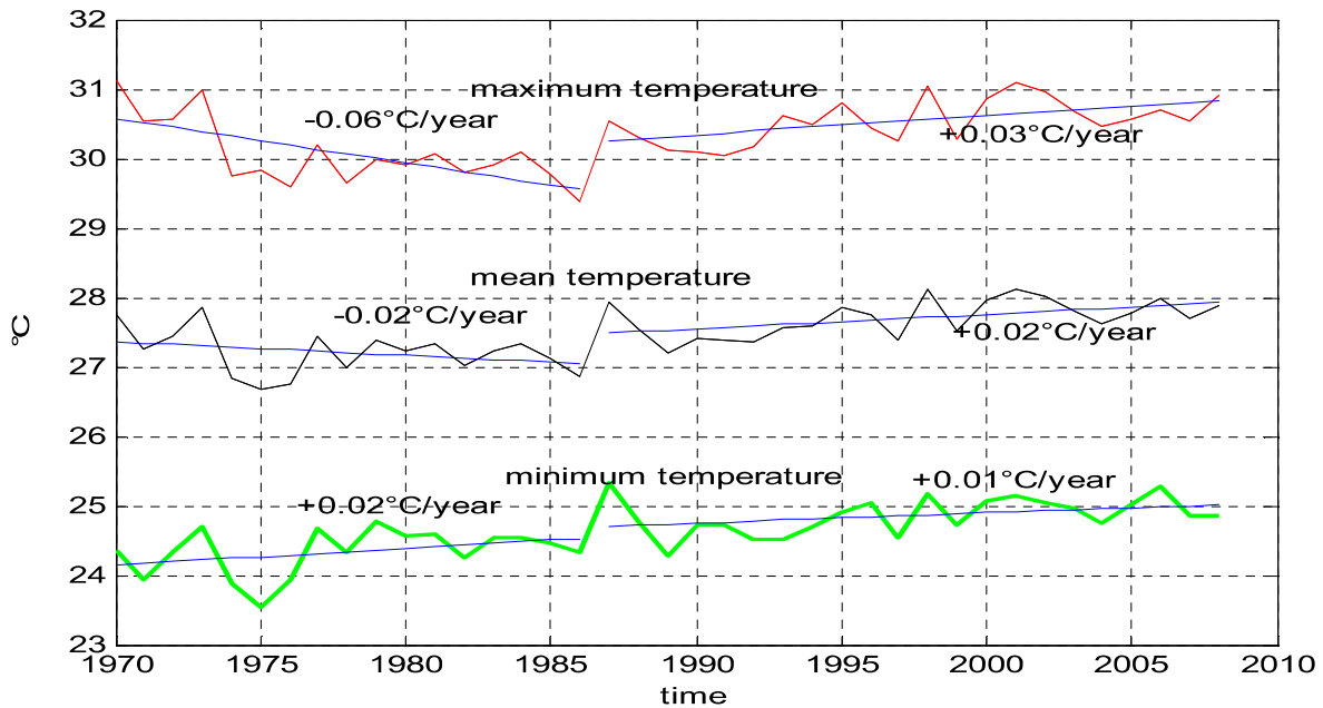
Fig. 1. Evolution of maximum and minimum temperatures in Cotonou
