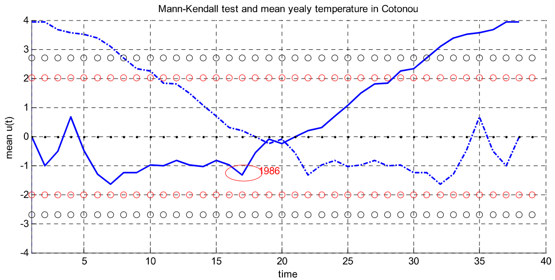
Fig. 4. The Kendall curves to determine trends
