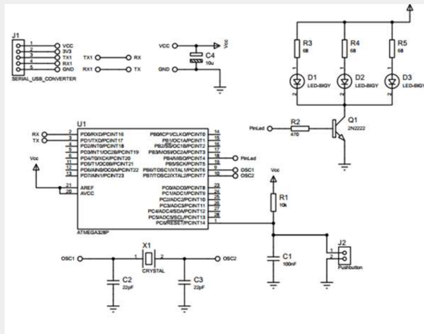
Figure 4: Emitter circuit of the designed LiFi prototype.
