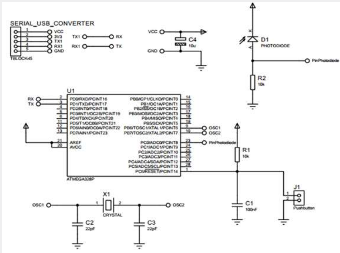
Figure 5: Receiver circuit of the designed LiFi prototype.
