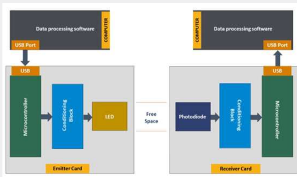
Figure 2: Bloc diagram concept of the LiFi prototype.
