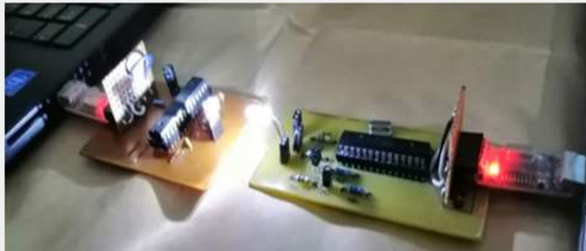
Figure 7: LiFi prototype connecting two computers for test.
