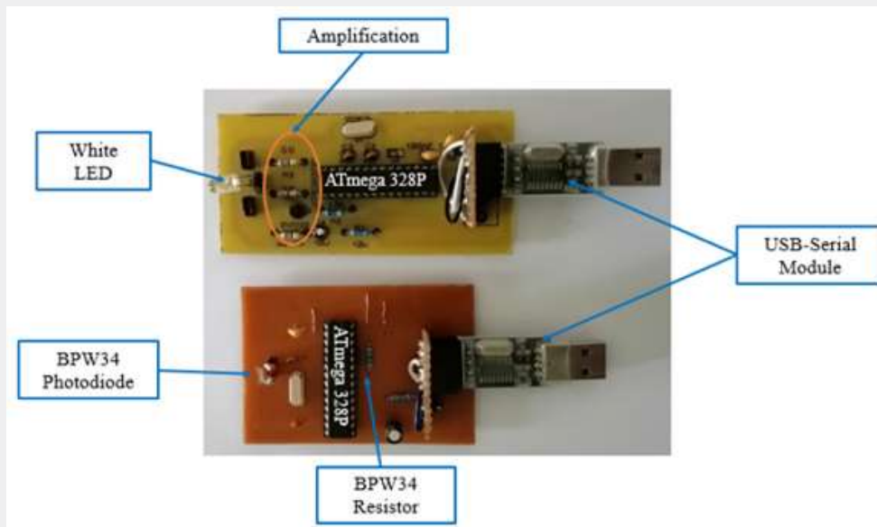
Figure 6: View of the designed LiFi prototype.
