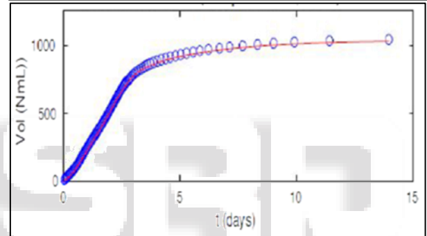
Fig. 3: Cumulative volume of biomethane obtained with the proposed model and that obtained by Mottelet et al. [17]
