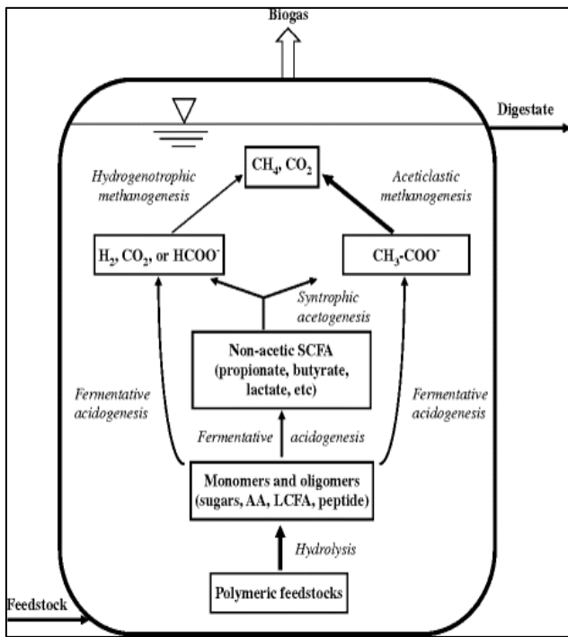
Fig. 1: Metabolic fluxes of anaerobic digestion [7].
