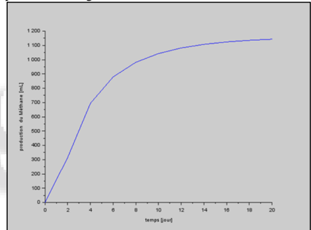
Fig. 2: Cumulative volume of biomethane.
