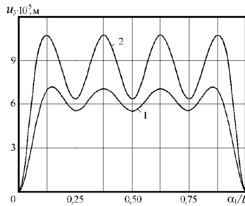
Fig. 4. Deflection variation curve u_3 according to coordinate \alpha_1
