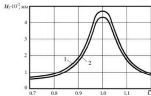
Fig. 5. Forced Vibration amplitudes with damping
