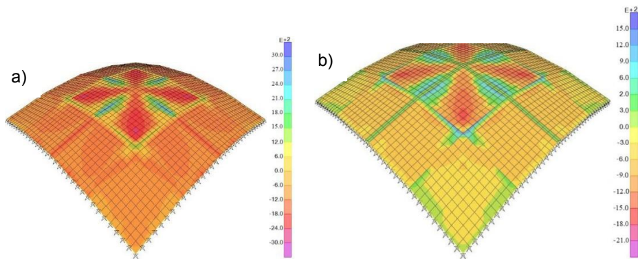
Fig. 9. Distribution of the dynamic stresses in the central section of folded shell
