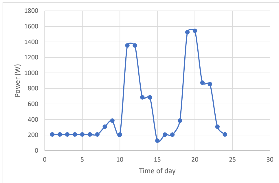
Fig. 5. Daily electricity load profile
