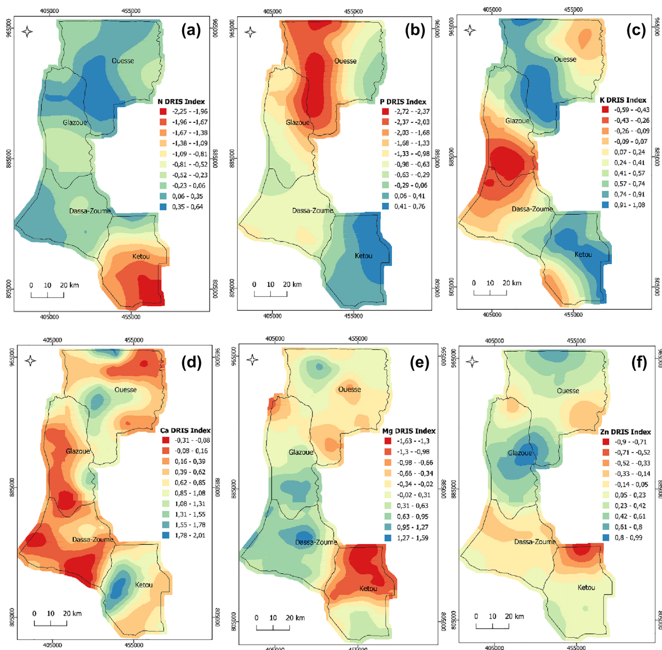
Figure 3. Spatial distribution maps of DRIS index of N (a), P (b), K (c), Ca (d), Mg (e), Zn (f).
