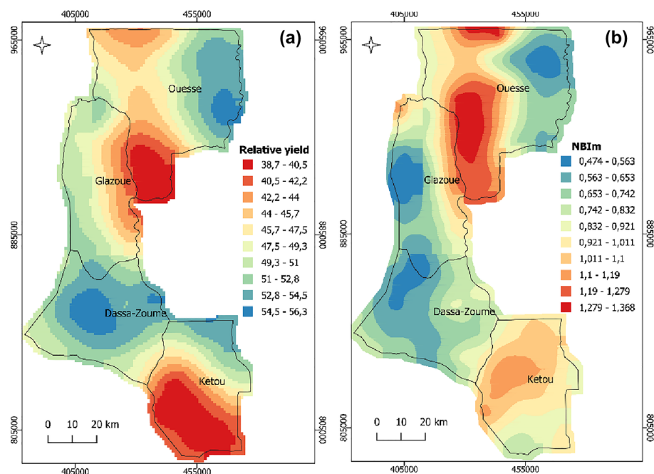
Figure 5. Spatial distribution maps of relative cowpea yield (a) and NBIm (b).
