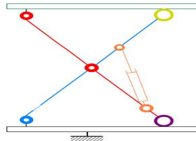
Fig. 5. 2D kinematic diagram of the lifting table
