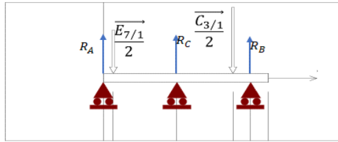
Fig. 11. Stresses on the side profile
