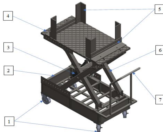
Fig. 1. Overview of the lifting table
