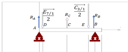
Fig. 12. Isostatic system
