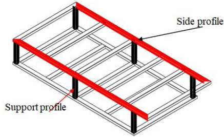
Fig. 10. Base structure
