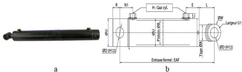
Fig. 13. (a) Double acting hydraulic cylinder. (b) Dimensions of the cylinder
