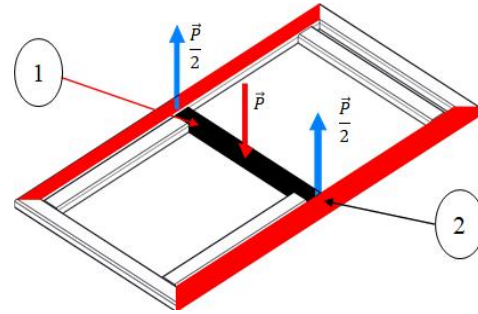
Fig. 6. Forces applied to the platform structure
