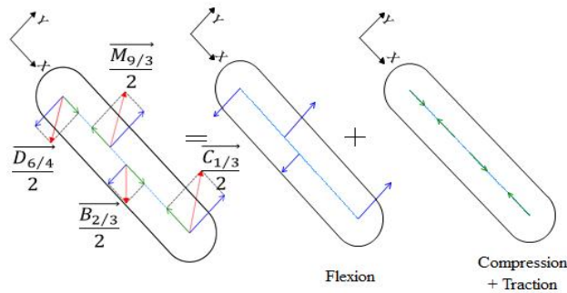
Fig. 9. Stresses on the scissors
