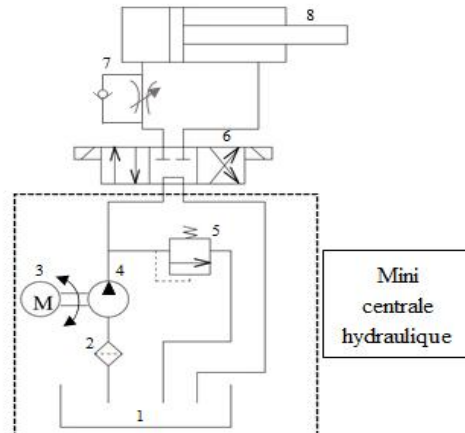
Fig. 15. Hydraulic circuit of the lifting table
