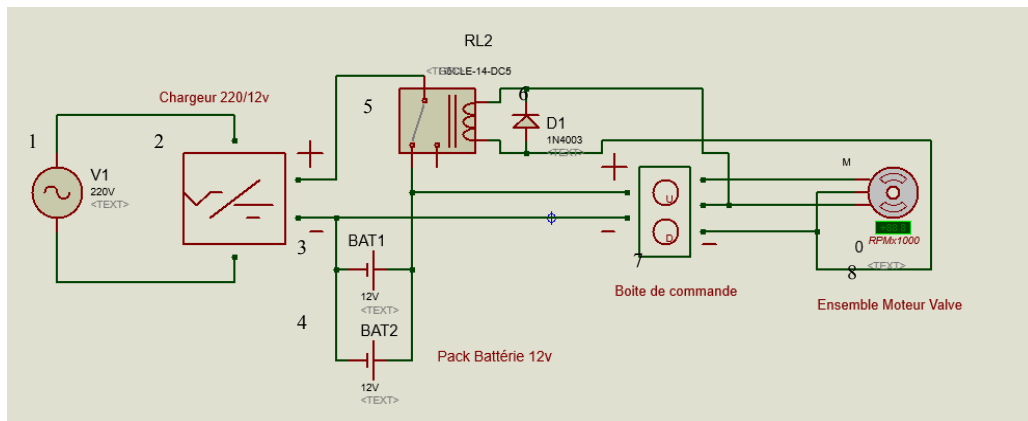
Fig. 17. Electrical circuit of the lifting table
