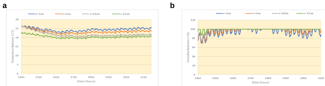
Fig. 12. Variation of temperature (a) and relative humidity (b) as a function of time over several layers in the chamber
