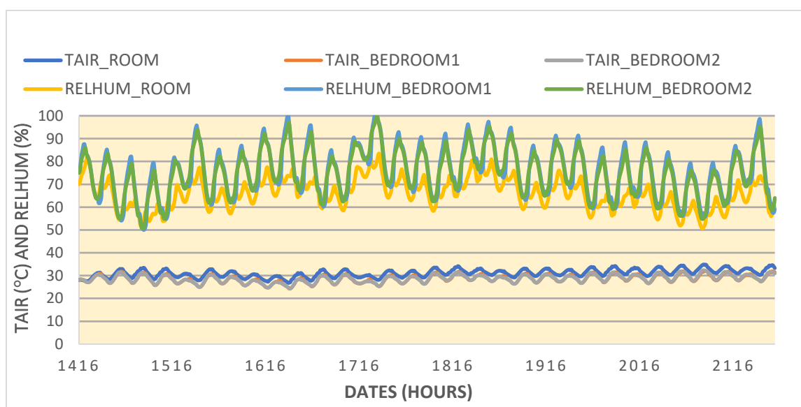
Fig. 7. Variation in relative humidity and temperature as a function of time in the living room, bedroom 1 and bedroom 2 over one month
