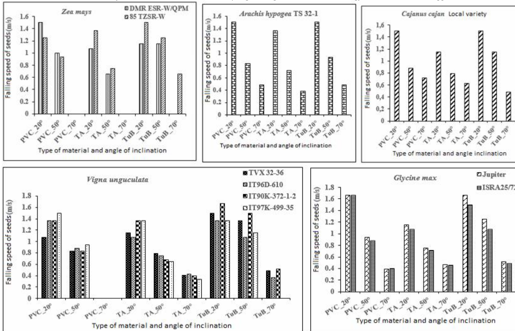
Fig. 1 Seed falling speed according to material type and angle of inclination
